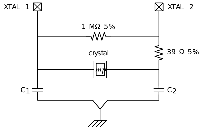
FIGURE 5-8: XTAL REFERENCE CLOCK
