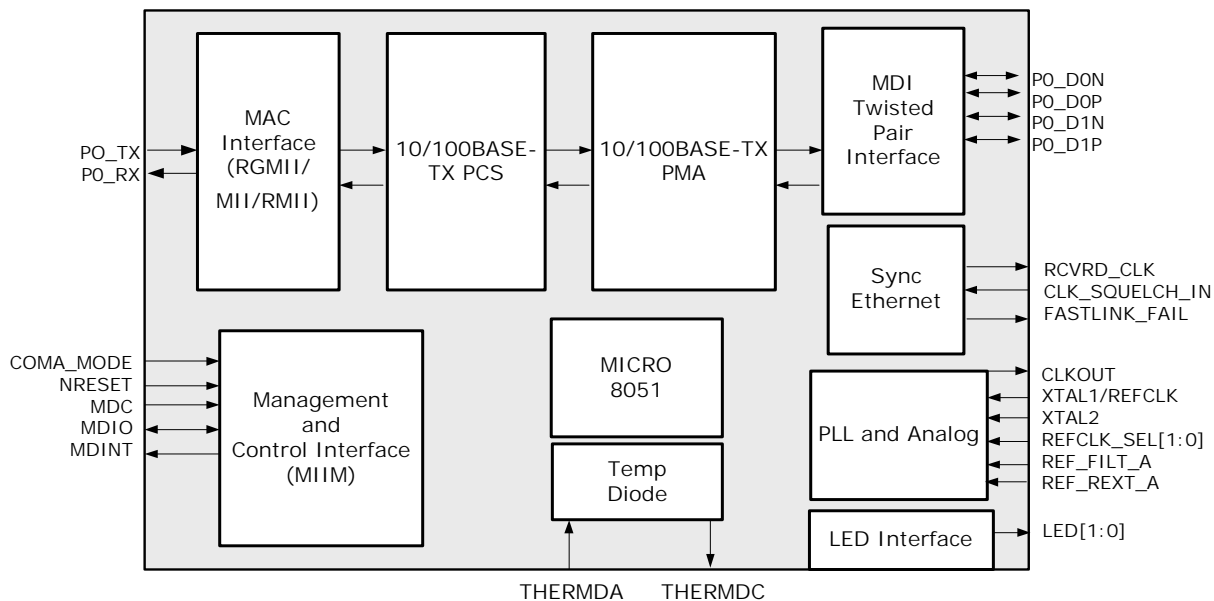
FIGURE 2-1: BLOCK DIAGRAM
