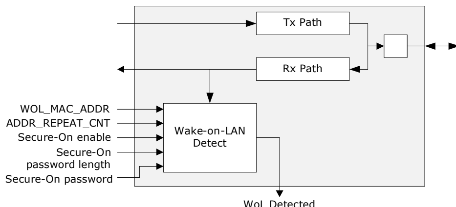
FIGURE 3-1: WAKE-ON-LAN FUNCTIONALITY
