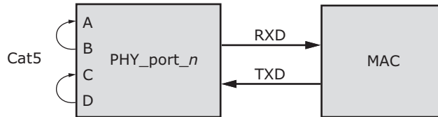
FIGURE 3-13: CONNECTOR LOOPBACK DIAGRAM
