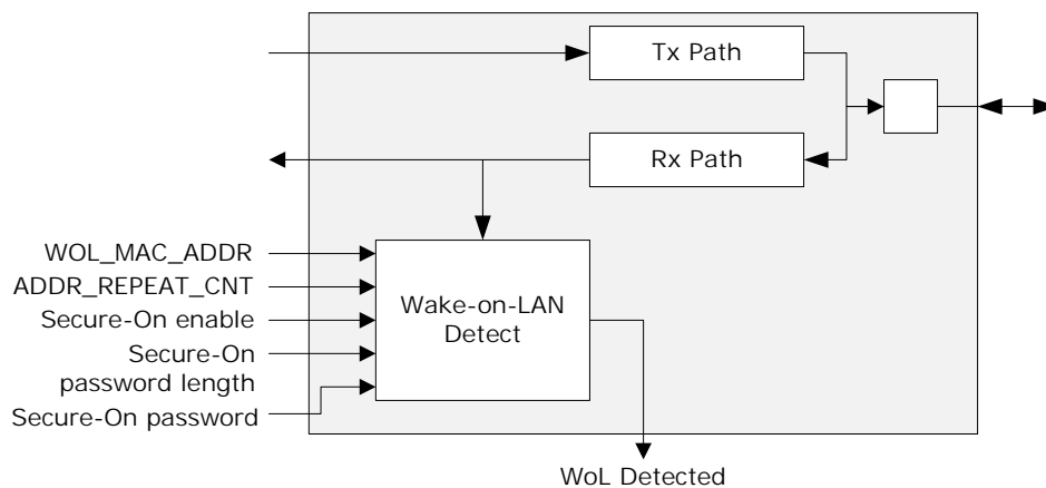
Figure 12 • Wake-On-LAN Functionality
