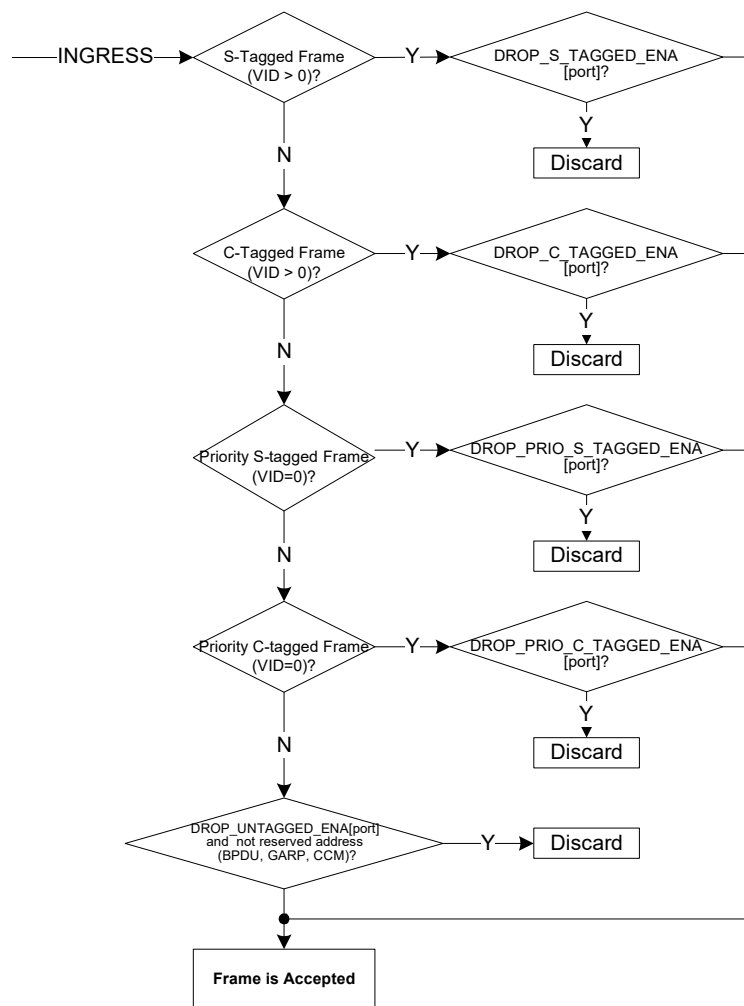
FIGURE 2-11: VLAN ACCEPTANCE FILTER
