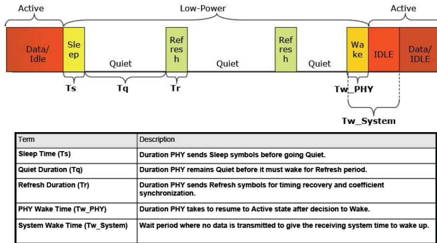
FIGURE 2-4: ENERGY EFFICIENT ETHERNET
