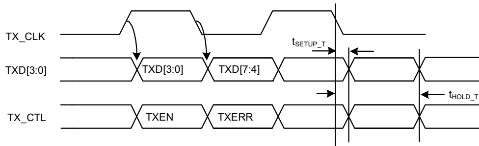
Figure 29 • Compensated Input RGMII Timing
