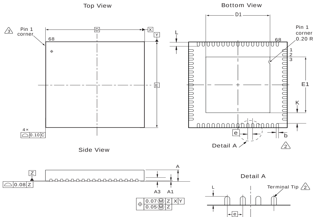
Figure 34 • Package Drawing
