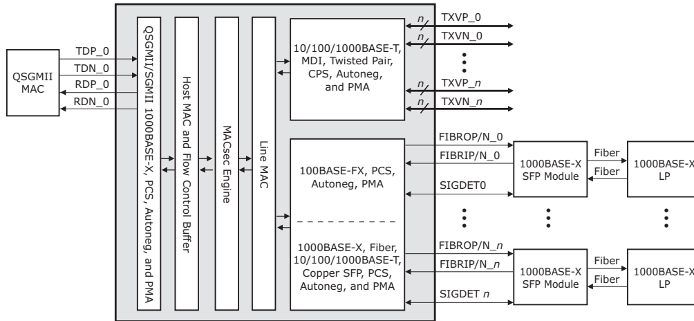
Figure 6 • QSGMII MAC to 100BASE-X Link Partner
