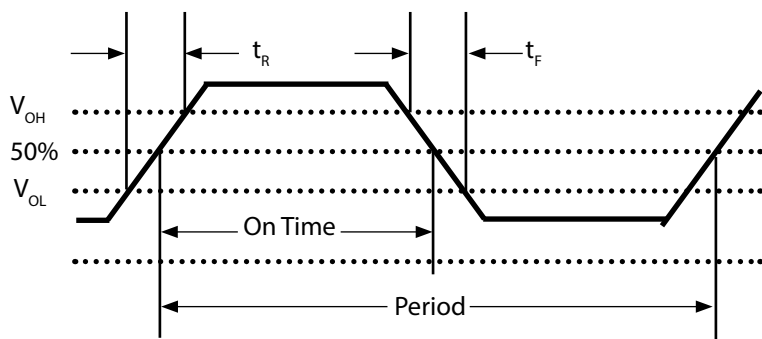
Fig 2: Waveform
