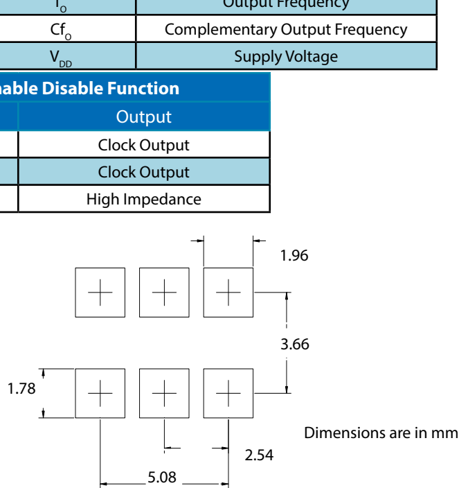
Figure 6. Pad Layout
