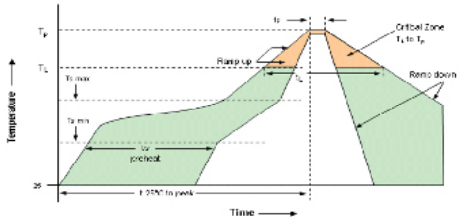
Solderprofile:
