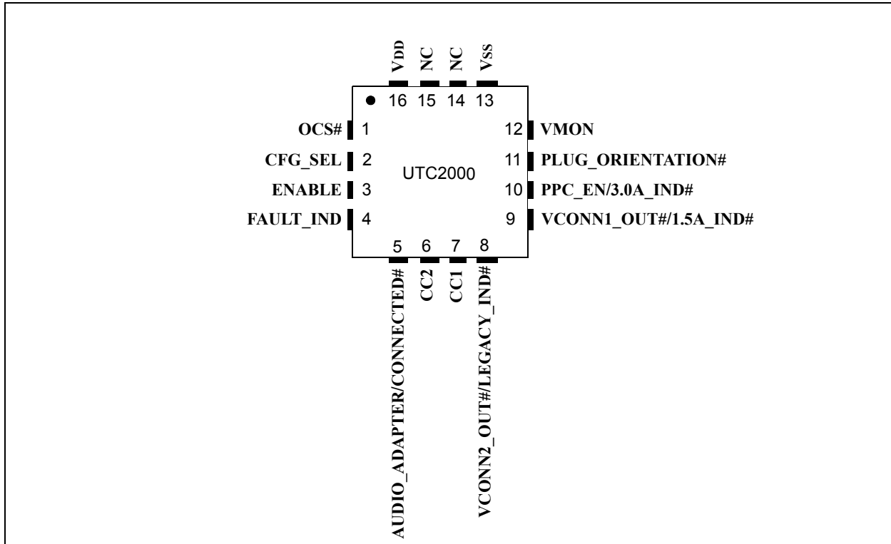
FIGURE 2-1: PIN ASSIGNMENTS
