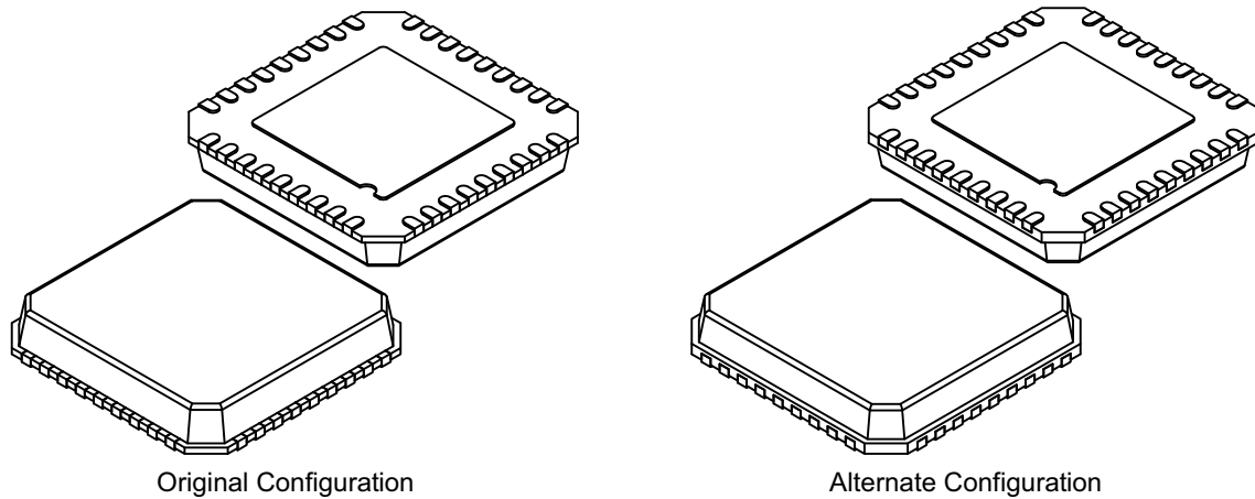
FIGURE 10-5: 36-QFN STANDARD PACKAGE (DIMENSIONS)
