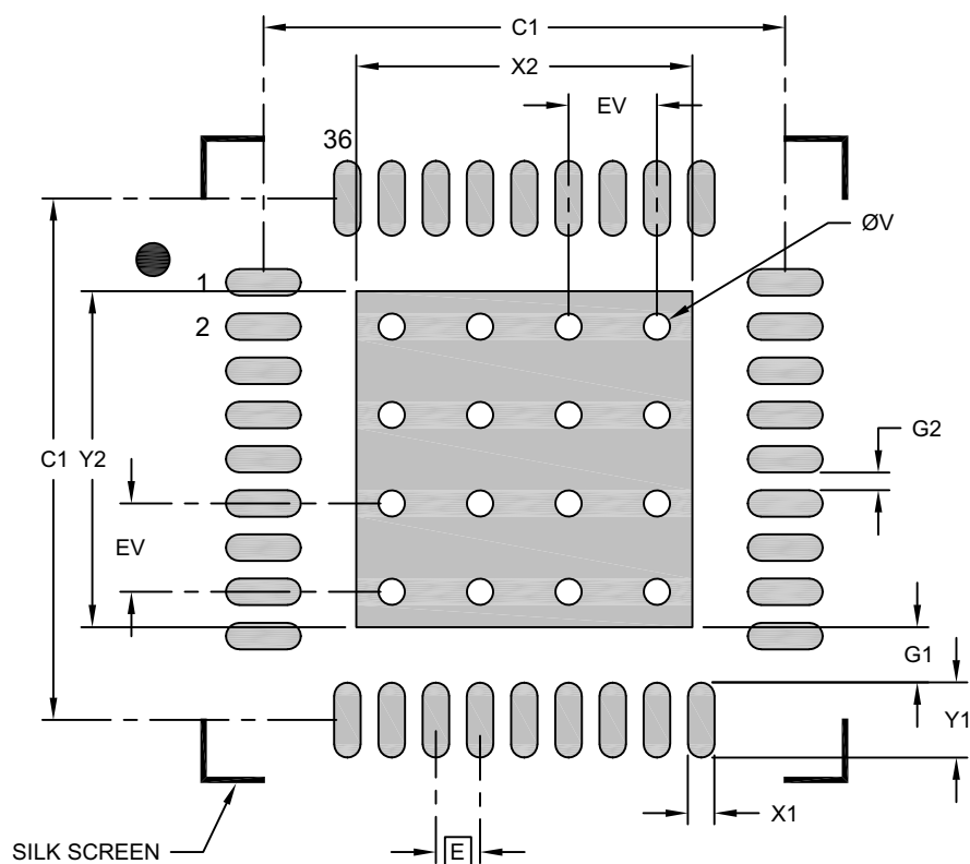
FIGURE 10-3: 36-QFN DIMPLE PACKAGE (LAND PATTERN)
