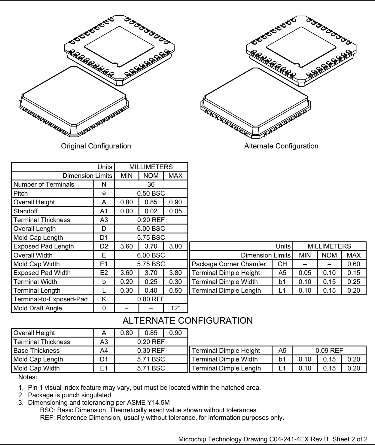
FIGURE 10-2: 36-QFN DIMPLE PACKAGE (DIMENSIONS)
