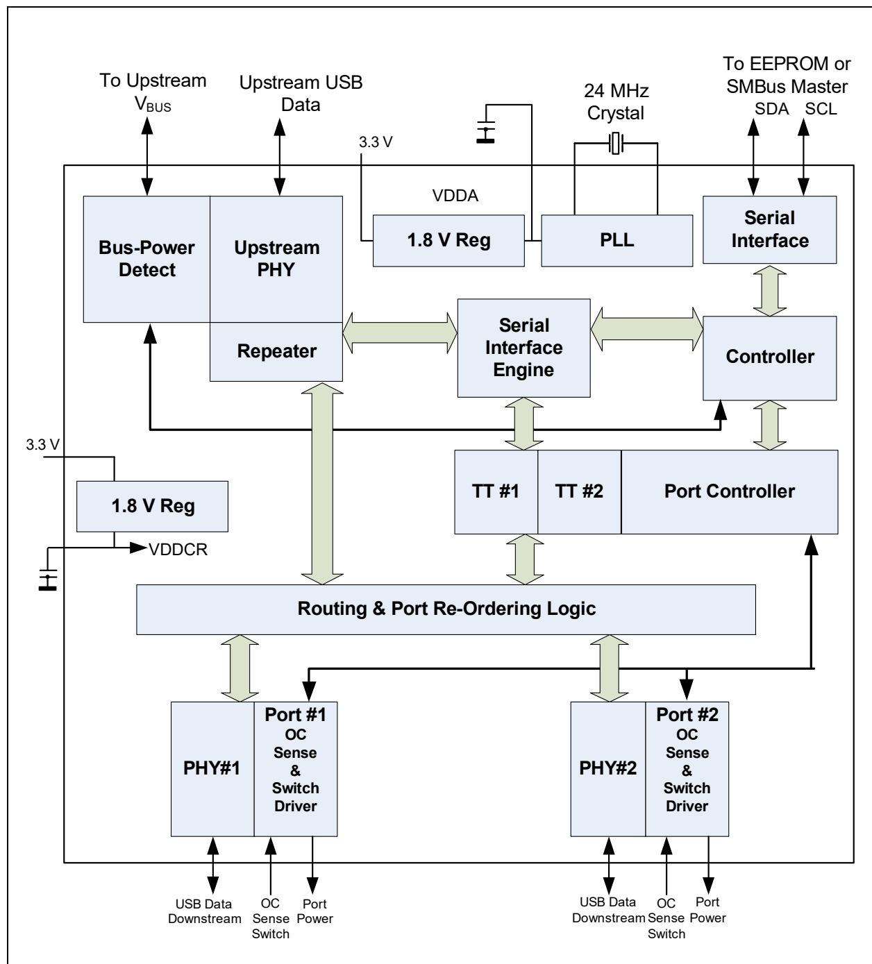
FIGURE 5-1: USB82512 BLOCK DIAGRAM
