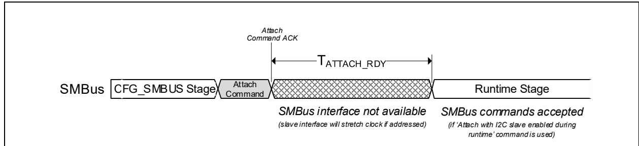
FIGURE 9-6: USB ATTACH COMMAND TO SMBUS SLAVE READY TIMING
