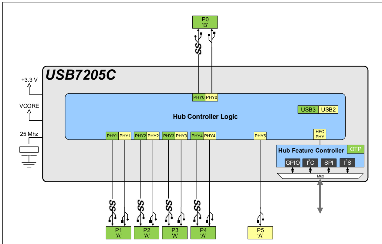
FIGURE 2-1: USB7205C INTERNAL BLOCK DIAGRAM - UPSTREAM TYPE- APPLICATION
