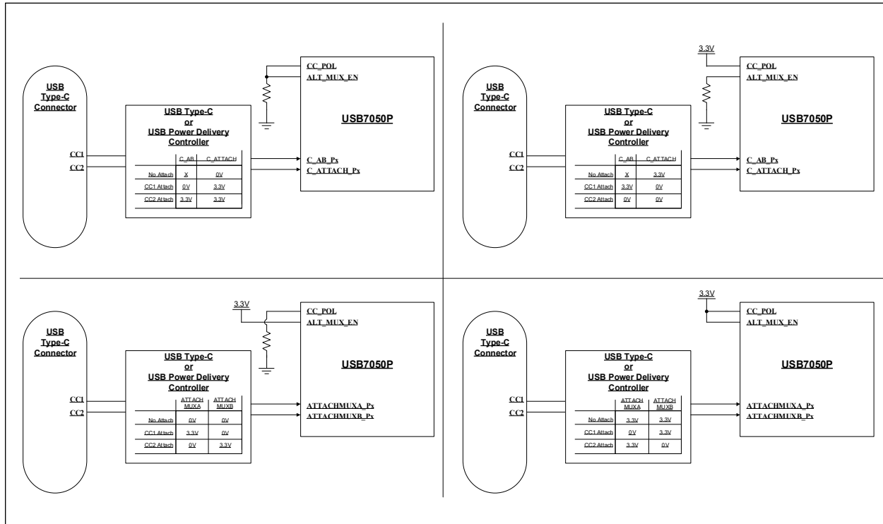
FIGURE 7-1: TYPE-C PORT CONTROL OPTIONS
