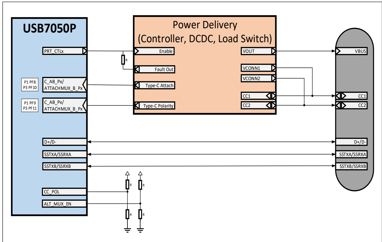
FIGURE 8-1: TYPICAL EXTERNAL USB POWER DELIVERY APPLICATION
