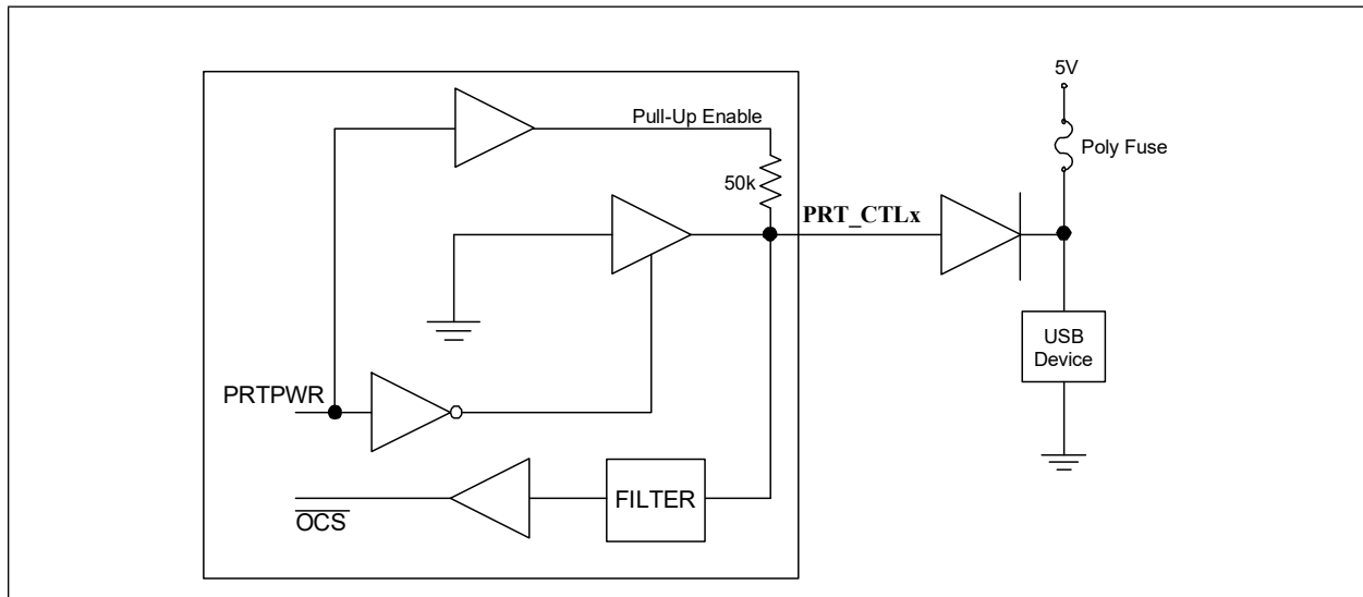
FIGURE 8-4: PORT POWER CONTROL USING A POLY FUSE
