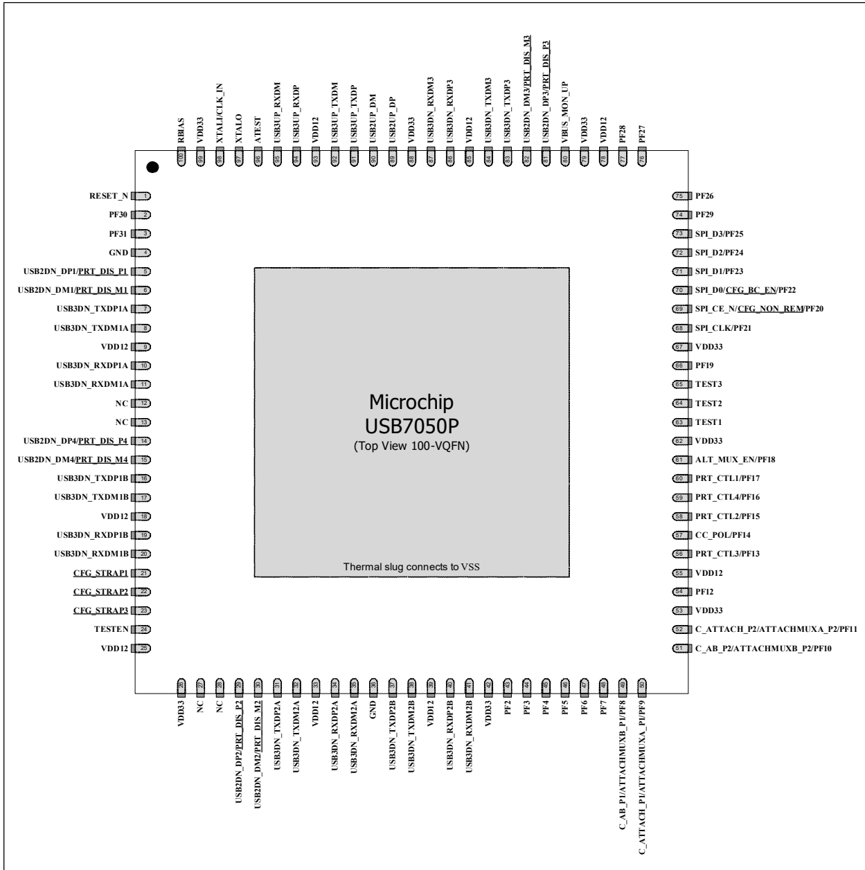
FIGURE 3-1: USB7050P 100-VQFN PIN ASSIGNMENTS
