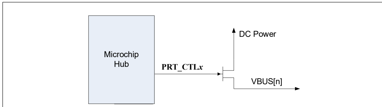
FIGURE 8-2: BATTERY CHARGING EXTERNAL POWER SUPPLY
