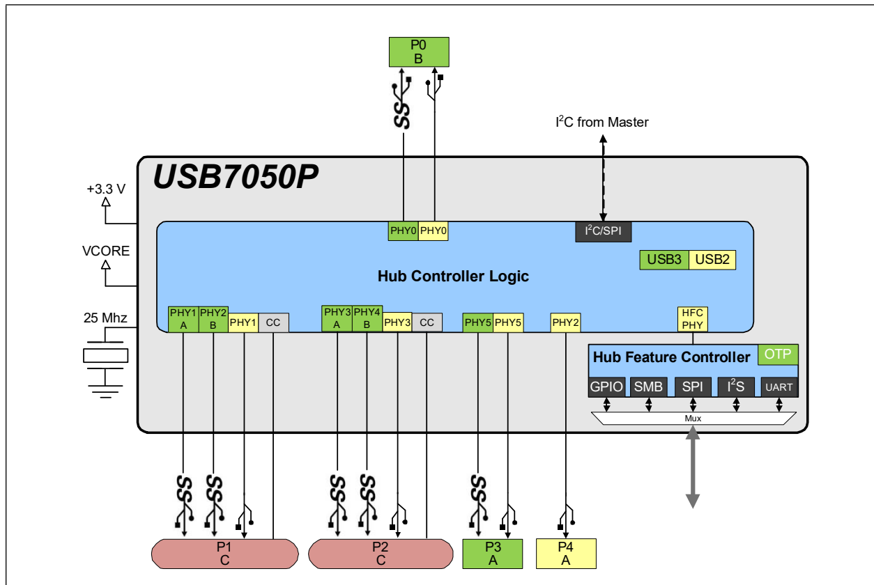
FIGURE 2-1: USB7050P INTERNAL BLOCK DIAGRAM - UPSTREAM TYPE-B APPLICATION
