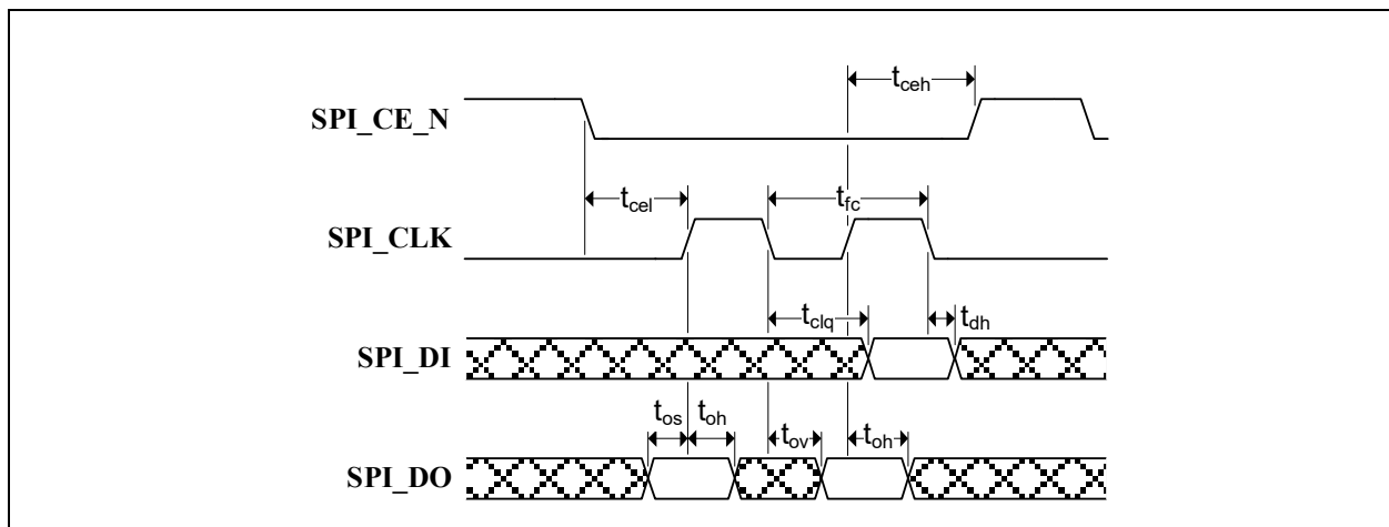
FIGURE 10-5: SPI TIMING
