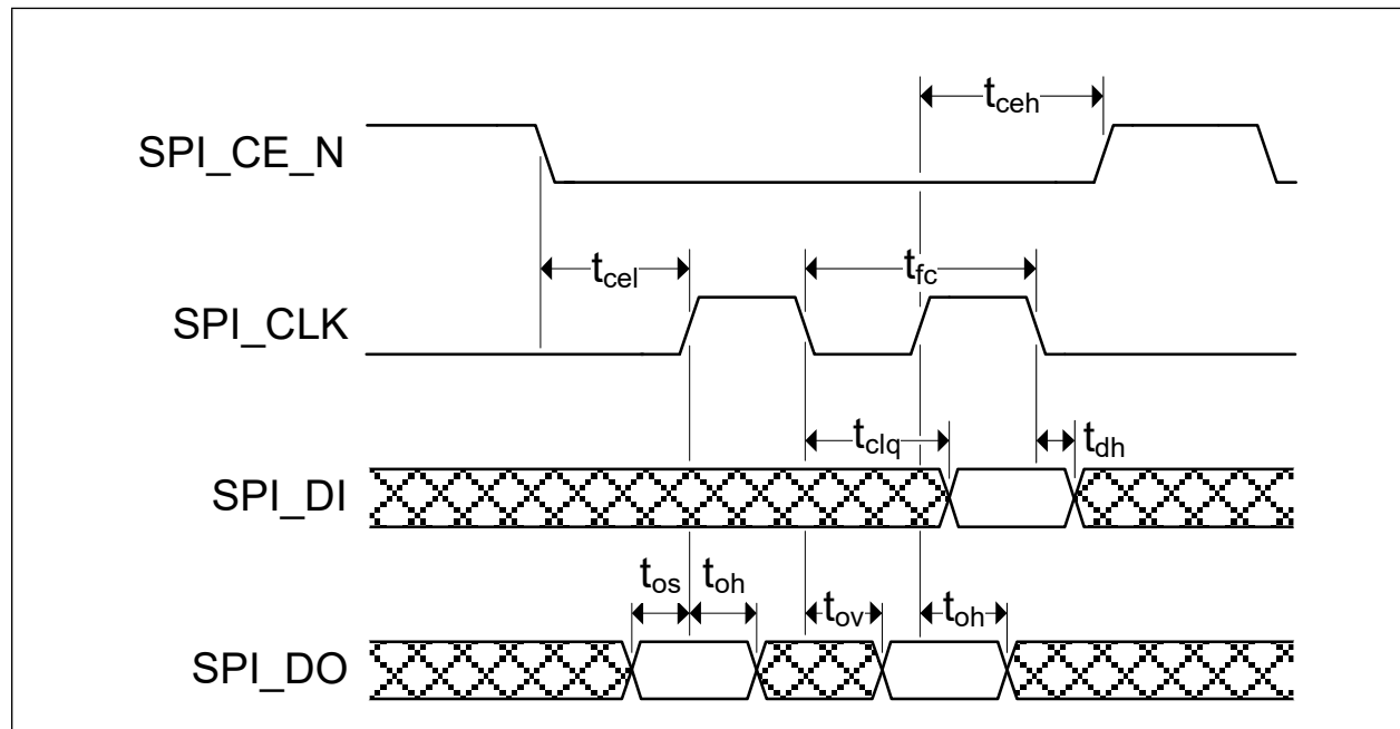
FIGURE 9-6: SPI TIMING
