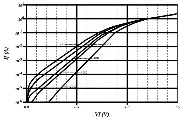
MEAN I_f VERSUS V_f CURVE VERSUS TEMPERATURE TYPICAL
