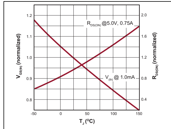
FIGURE 2-11: V_{(th)} and R_{DS(ON)} with Temperature.
