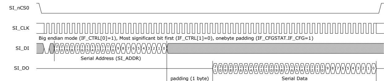
FIGURE 3-7: READ SEQUENCE FOR ONE-BYTE PADDING
