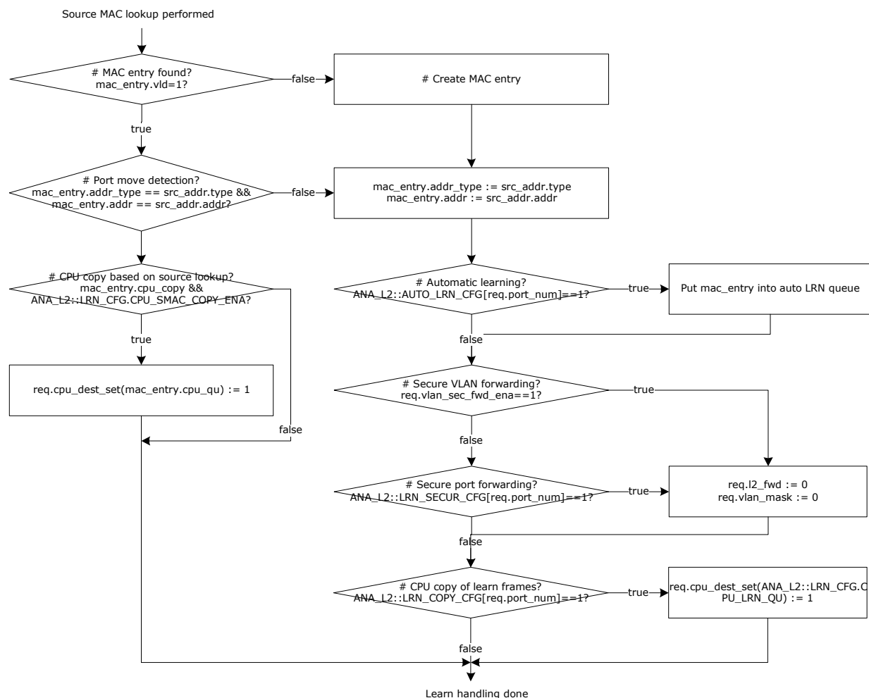
FIGURE 2-29: SOURCE CHECK
