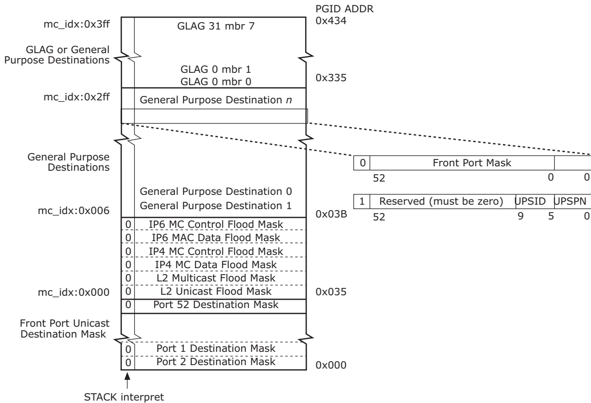
FIGURE 2-30: PGID LAYOUT
