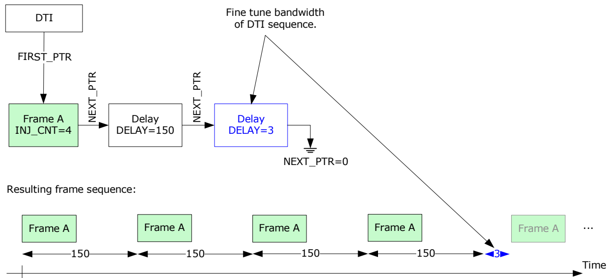
FIGURE 2-62: FINE TUNING BANDWIDTH OF DTI SEQUENCE
