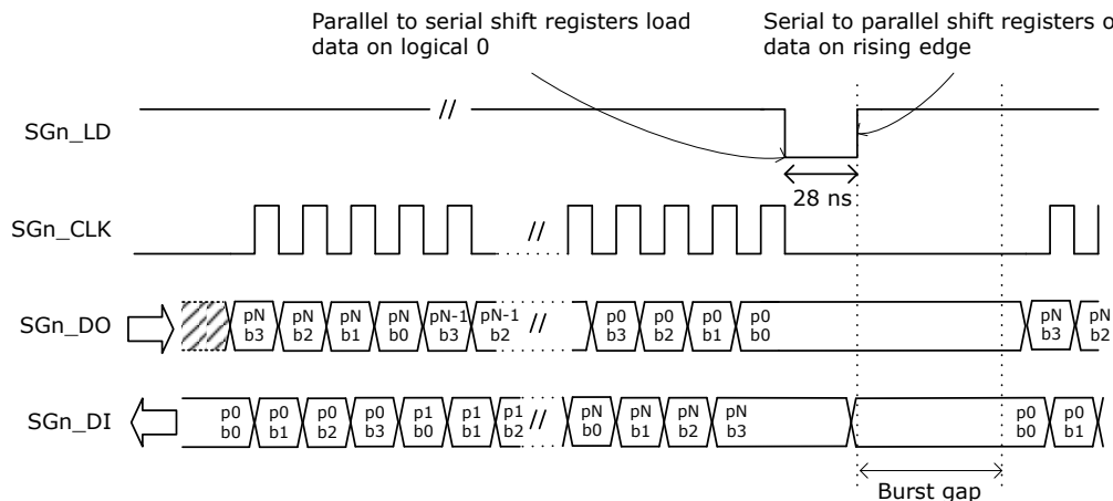
Figure 5-25. SIO Timing
