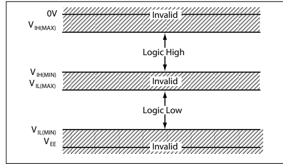
FIGURE 7-5: Input Levels, NECL.
