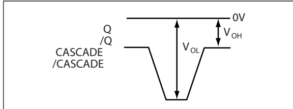
FIGURE 7-2: Output Levels, NECL.
