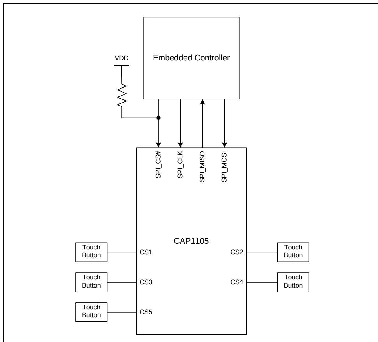
Figure 4.2 System Diagram for CAP1105
