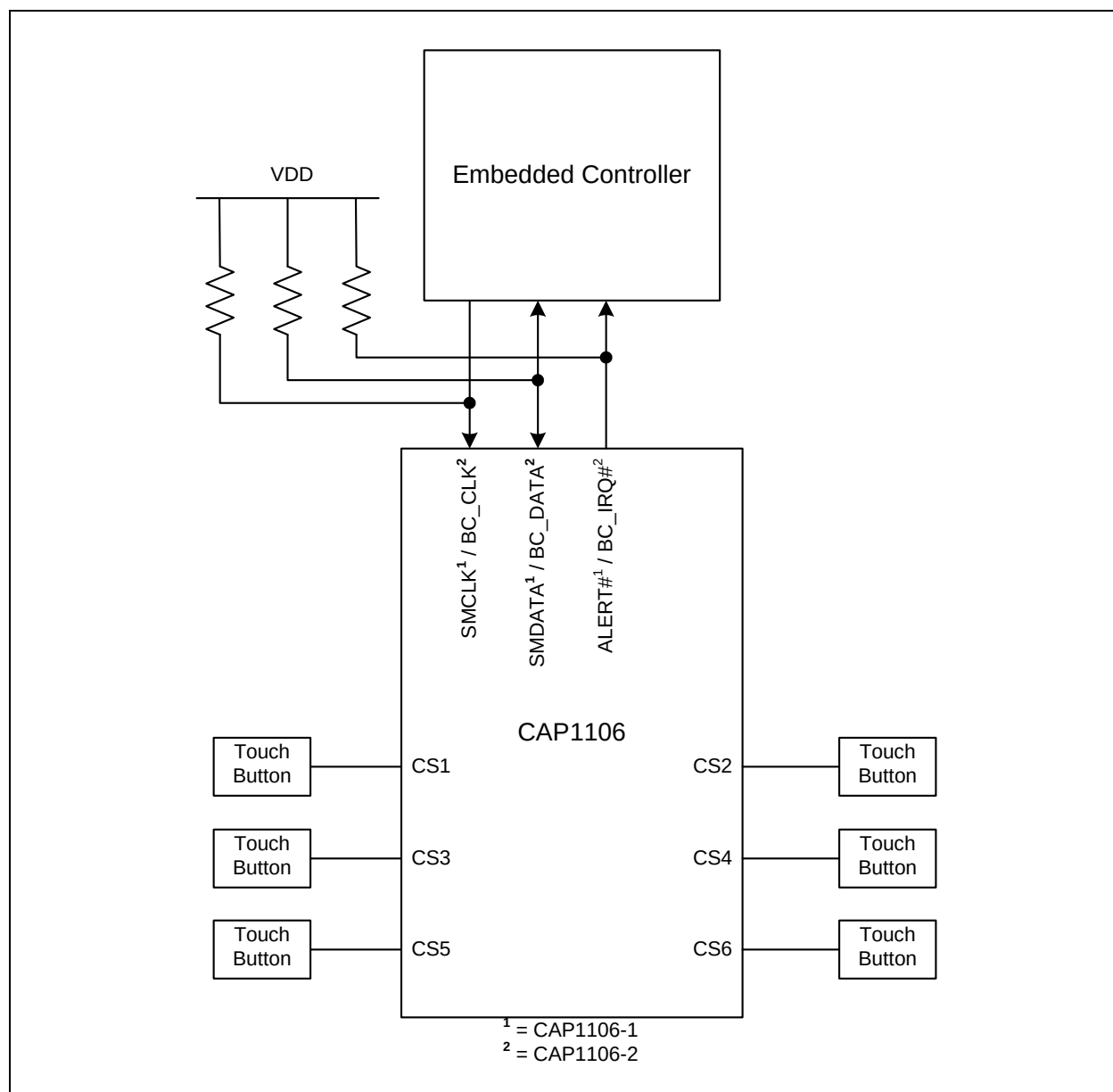
Figure 4.1 System Diagram for CAP1106
