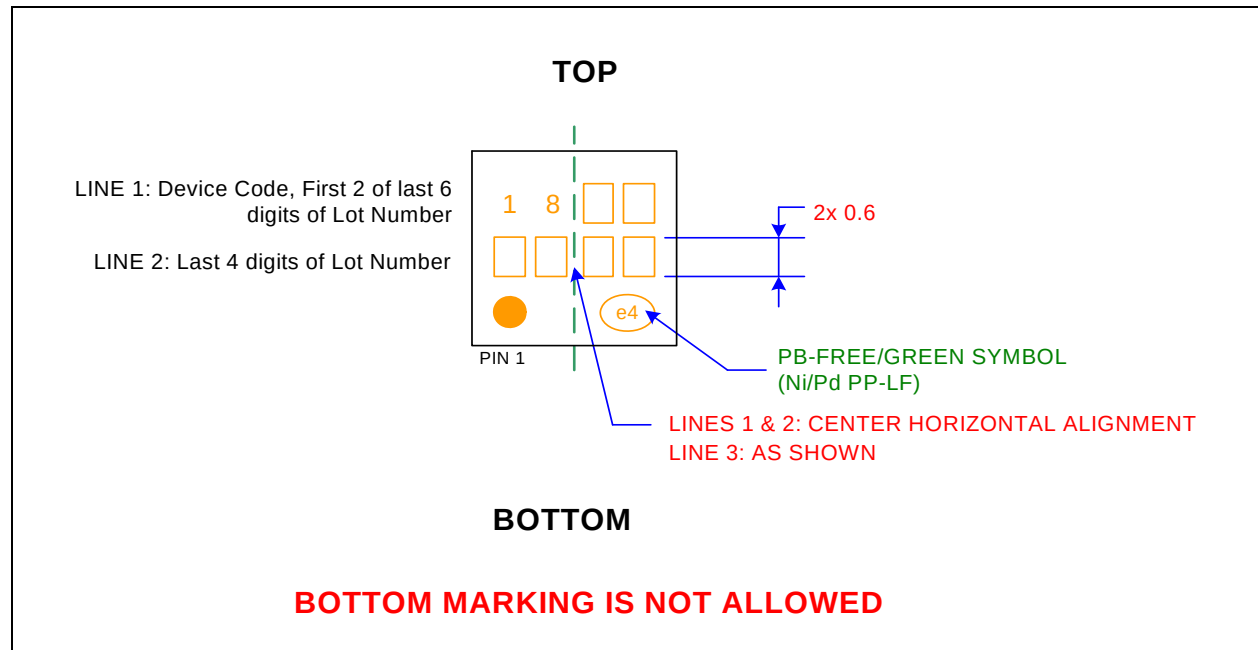
Figure 6.4 CAP1106-1 Package Markings
