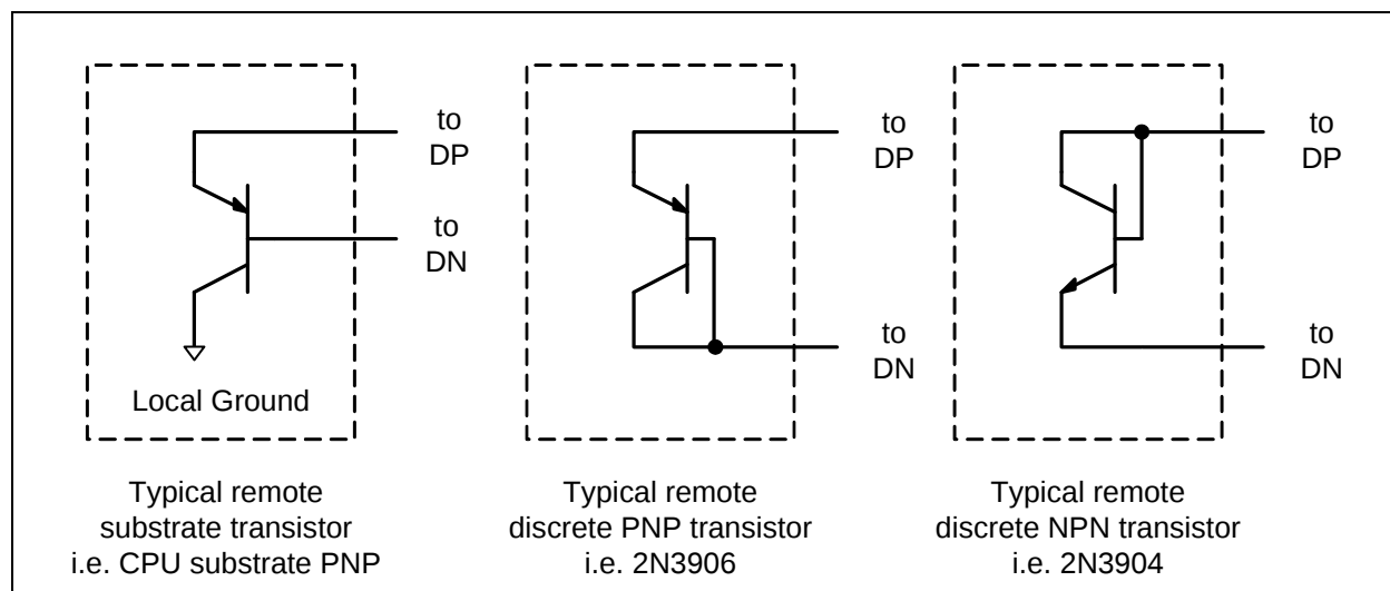
Figure 4.2 Diode Connections
