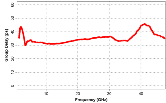
Group Delay
