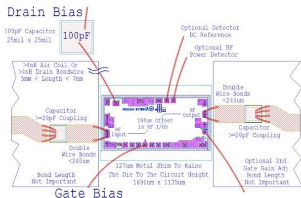
30GHz bonding diagram
