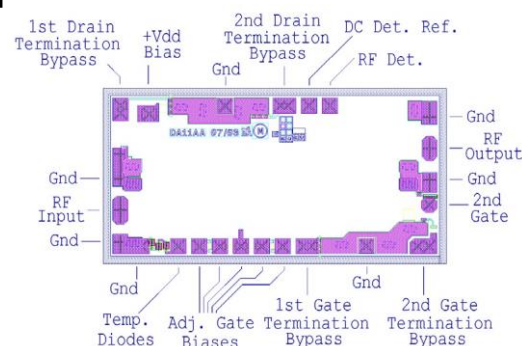
40MHz - 30GHz bonding diagram
