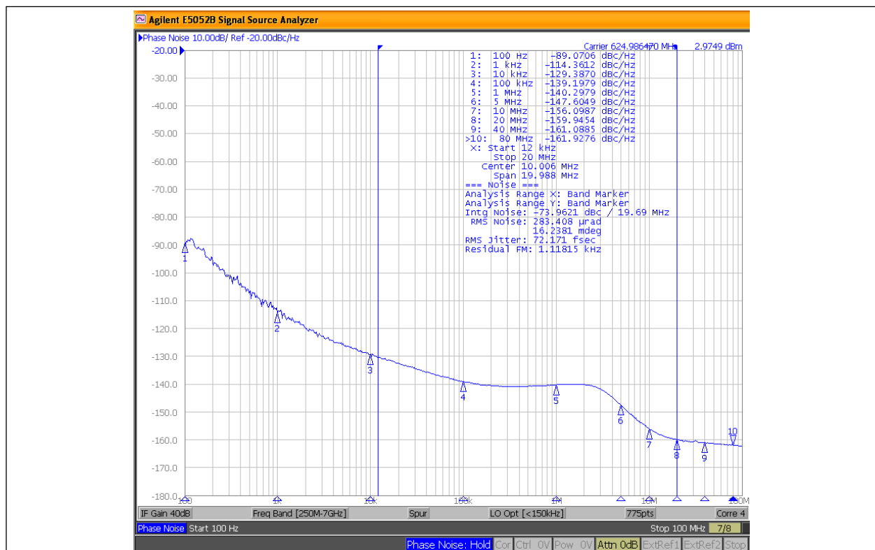
FIGURE 7-4: 625.0000 MHz, Integration Range 12 kHz to 20 MHz: 72.1 f RMS .
