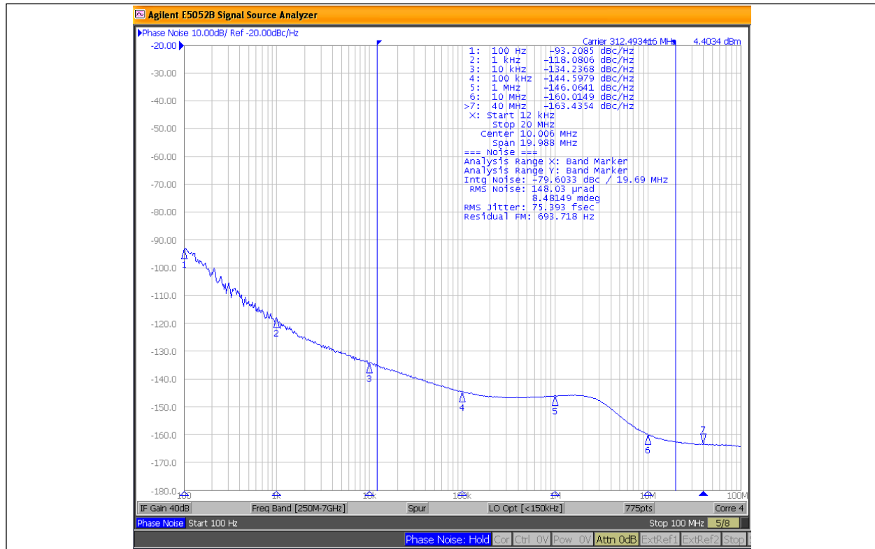
FIGURE 7-3: 312.500 MHz, Integration Range 12 kHz to 20 MHz: 75.4 f RMS .
