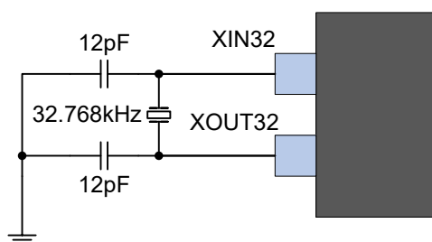
Figure 47-10. External Real Time Oscillator with Load Capacitor
