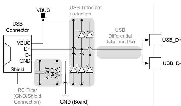
Figure 47-17. Protected USB Interface Example Schematic
