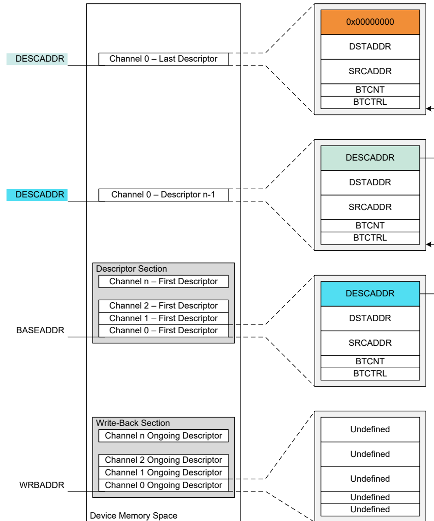
Figure 25-3. Memory Sections
