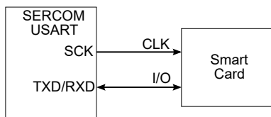
Figure 31-15. Connection of a Smart Card to the SERCOM USART
