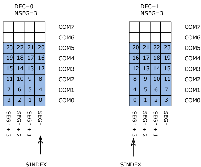
Figure 42-24. Character Mapping Order
