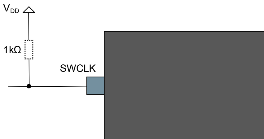
Figure 47-12. SWCLK Circuit Connections
