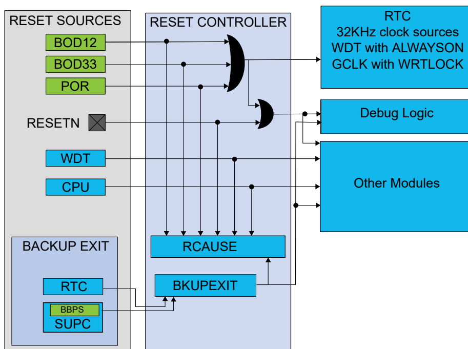
Figure 18-1. Reset System
