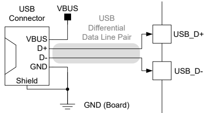
Figure 47-16. Low Cost USB Interface Example Schematic
