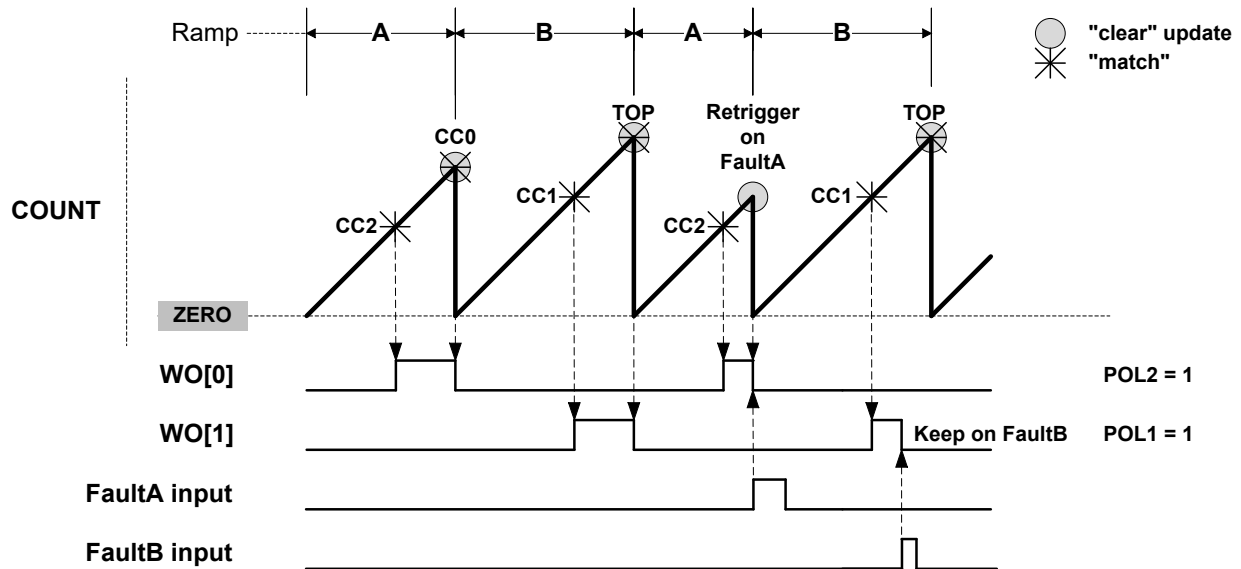
Figure 35-20. RAMP2 Critical Operation With More Than 2 Channels
