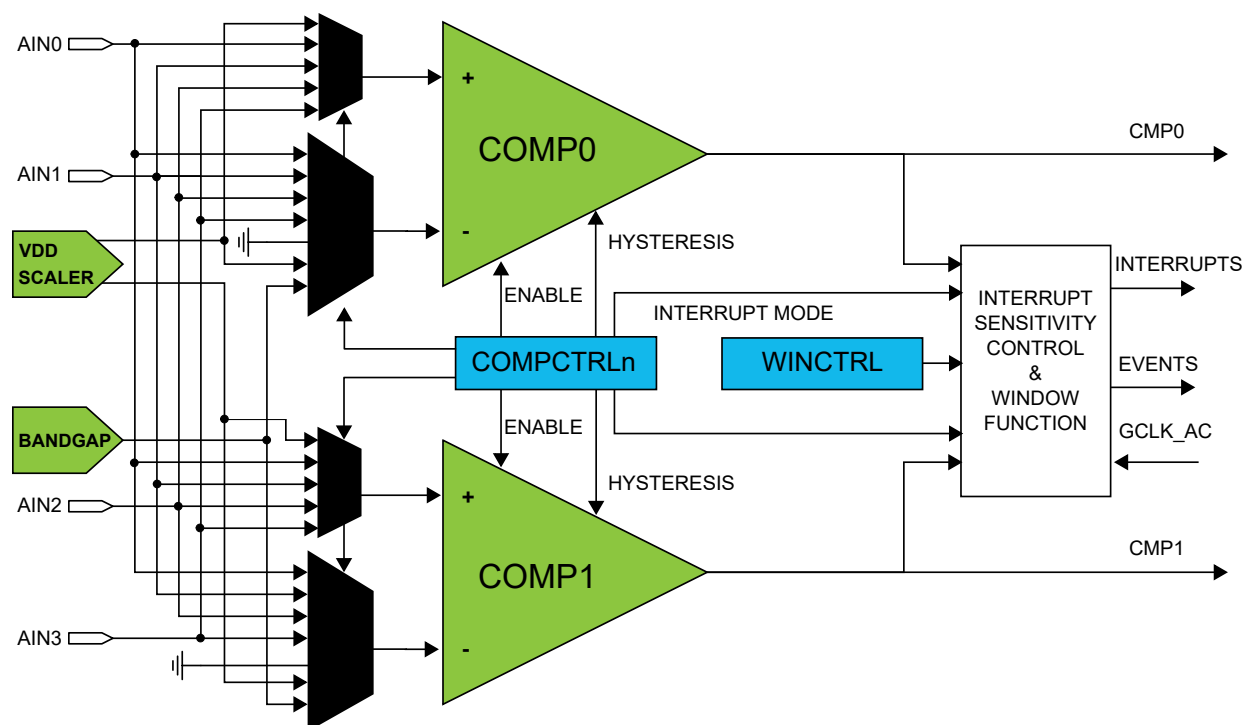
Figure 41-1. Analog Comparator Block Diagram
