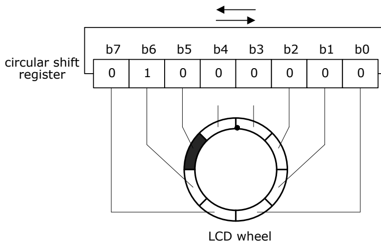
Figure 42-20. LCD Wheel Animation Example (8 Segments)
