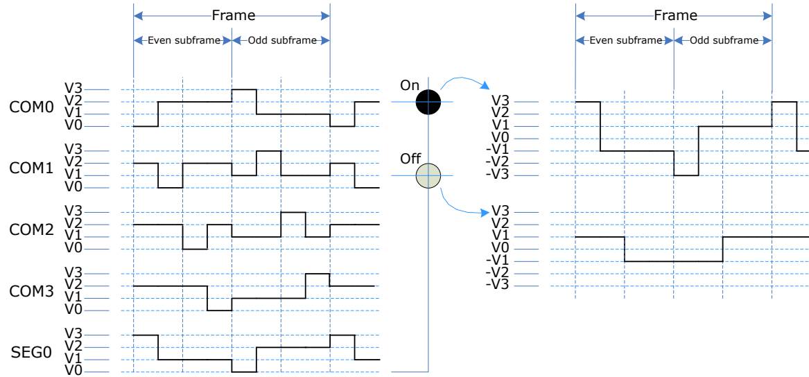
Figure 42-12. 1/3 Bias, 1/4 Duty, Low-Power Waveform
