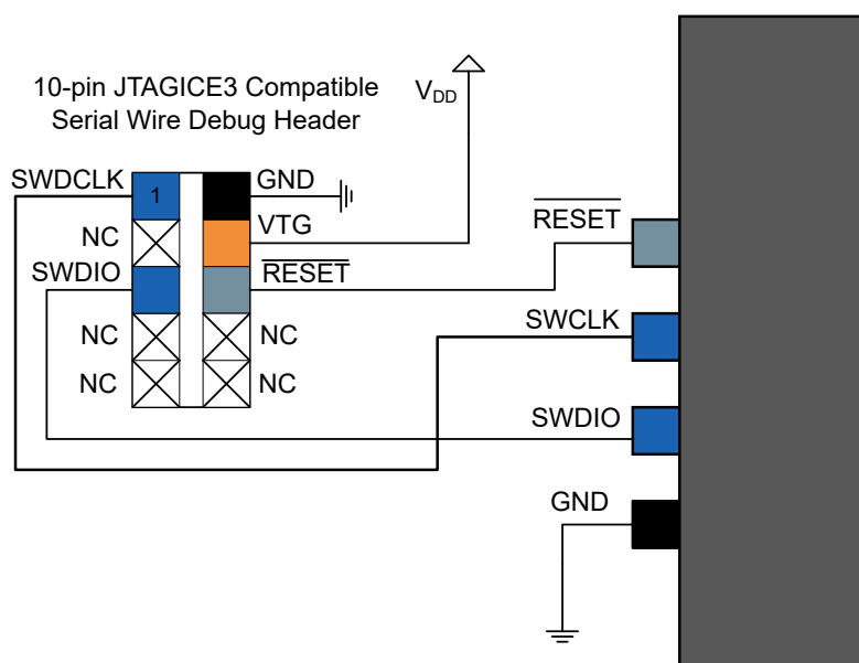
Figure 47-14. 10-pin JTAGICE3 Compatible Serial Wire Debug Interface
