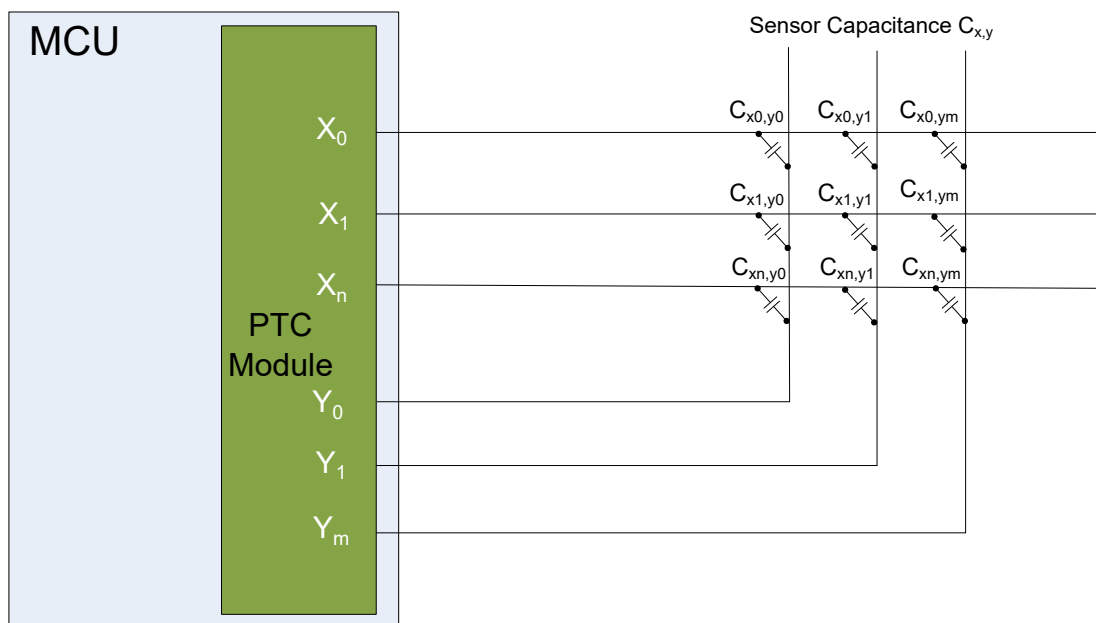
Figure 43-3. Mutual Capacitance Sensor Arrangement
