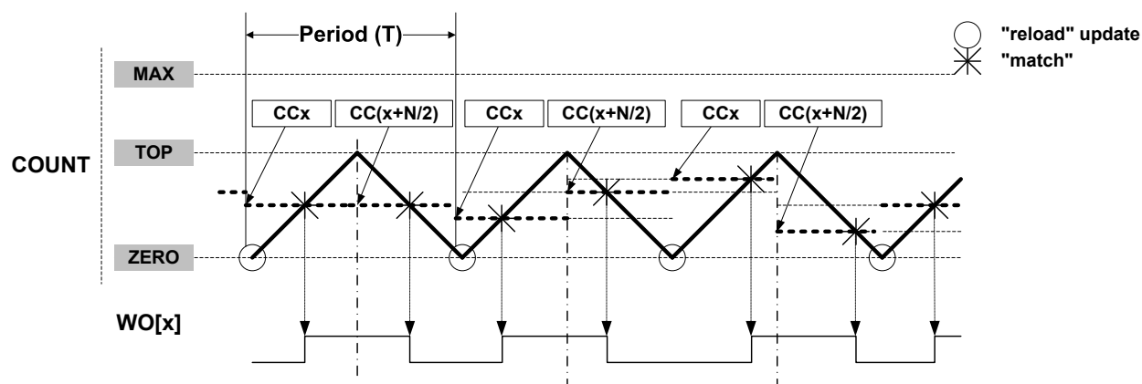
Figure 35-8. Dual-Slope Critical Pulse Width Modulation ( N=\text{CC\_NUM} )
