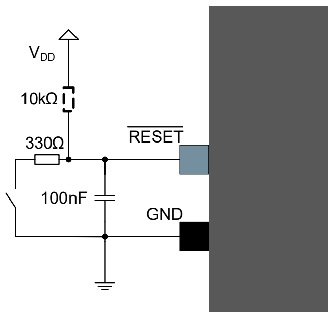
Figure 47-6. External Reset Circuit Schematic
