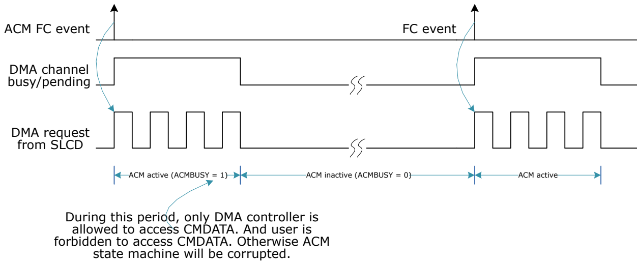
Figure 42-29. Limitations of Auto Character Mapping Mode
