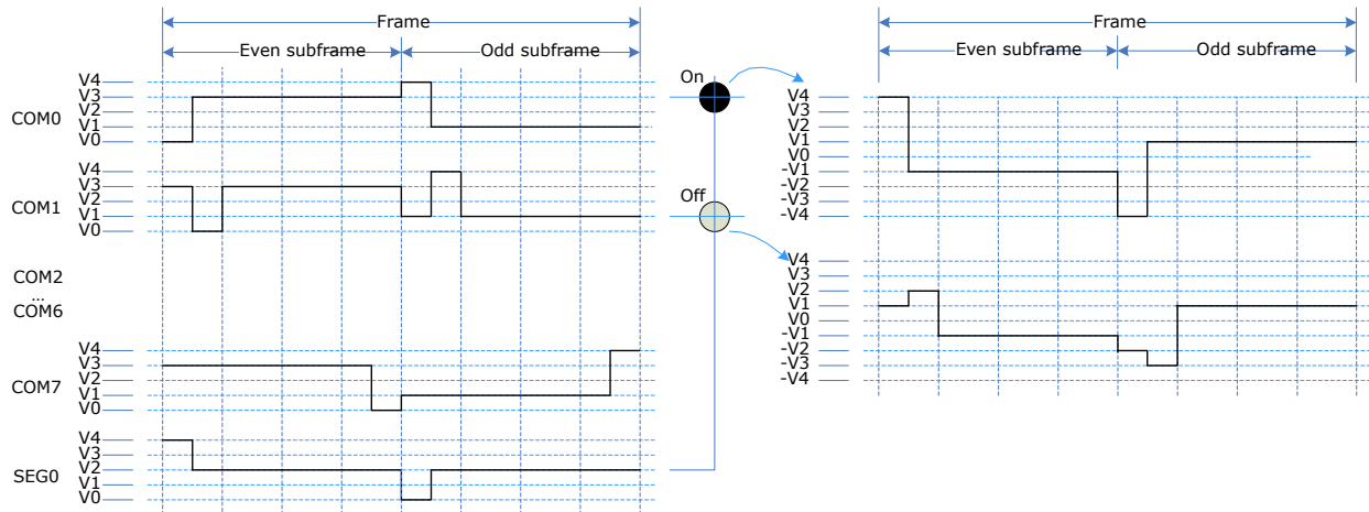
Figure 42-15. 1/4 Bias, 1/8 Duty, Low-Power Waveform
