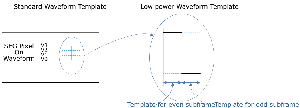
Figure 42-8. Derive Low-Power Waveform Template from Standard Waveform Template
