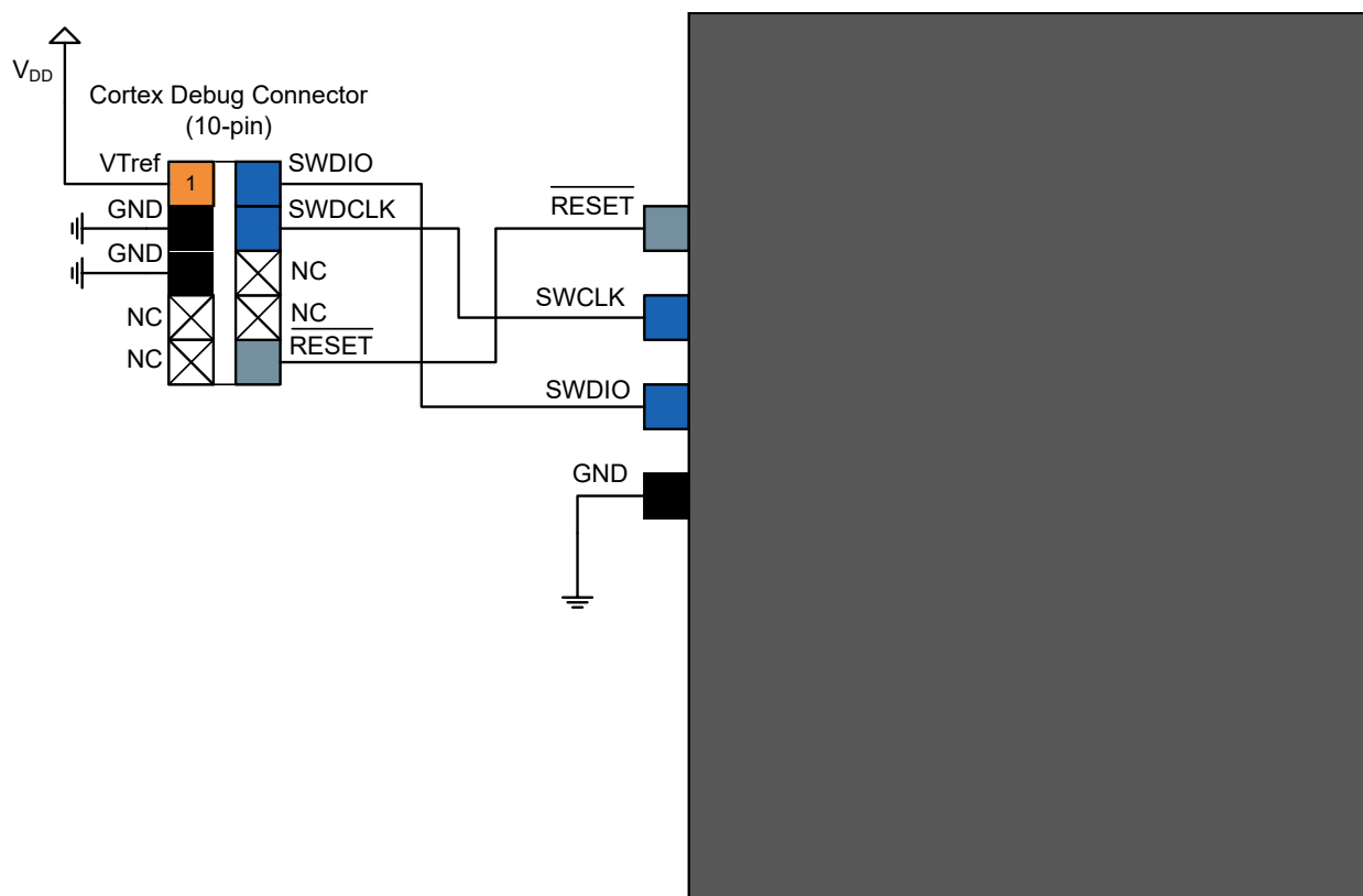
Figure 47-13. Cortex Debug Connector (10-pin)
