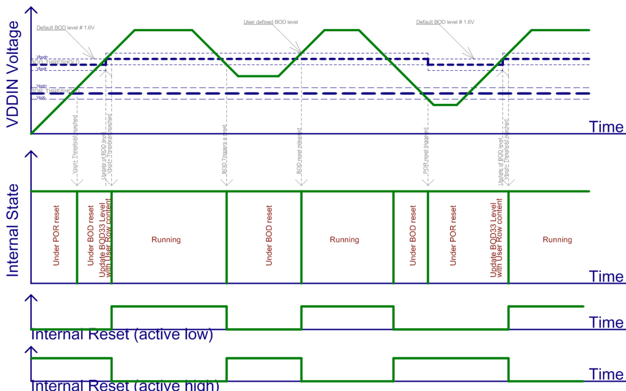
Figure 44-1. BOD Reset Behavior at Startup and Default Levels
