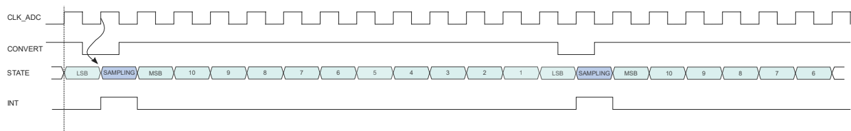
Figure 40-6. ADC Timing for Free Running in 12-bit Resolution
