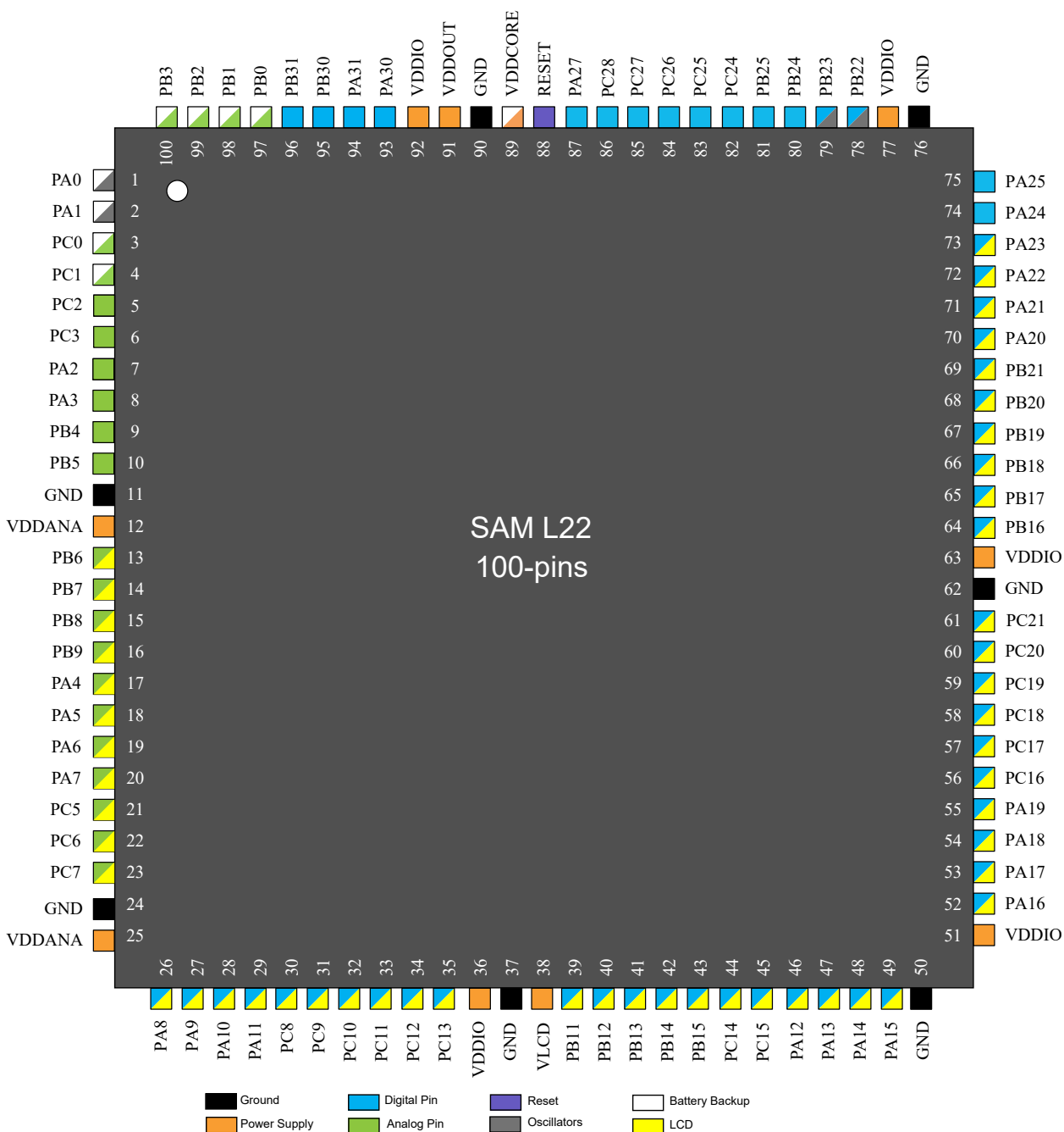
Figure 4-3. TQFP100
