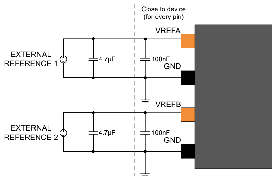
Figure 47-4. External Analog Reference Schematic With Two References
