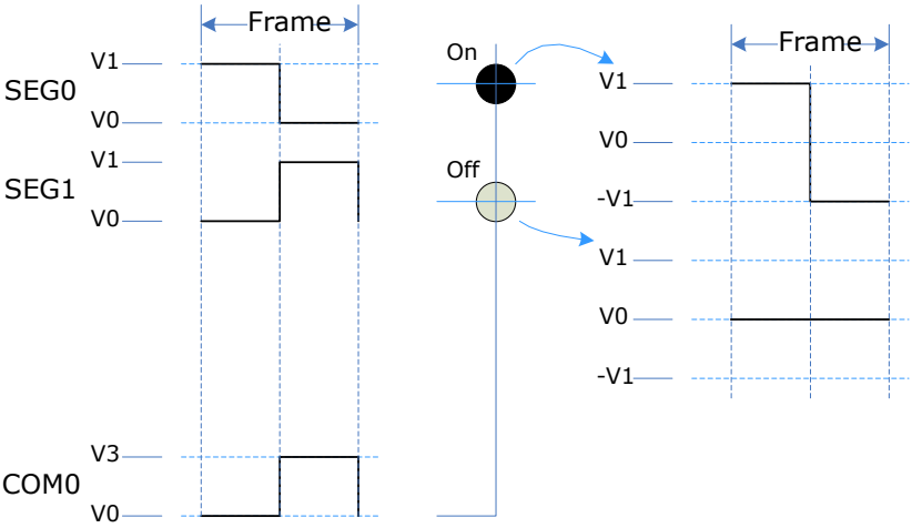
Figure 42-5. Static Bias and Duty Waveform
