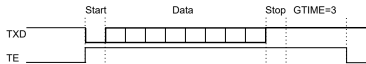
Figure 31-14. Example of TE Drive with Guard Time
