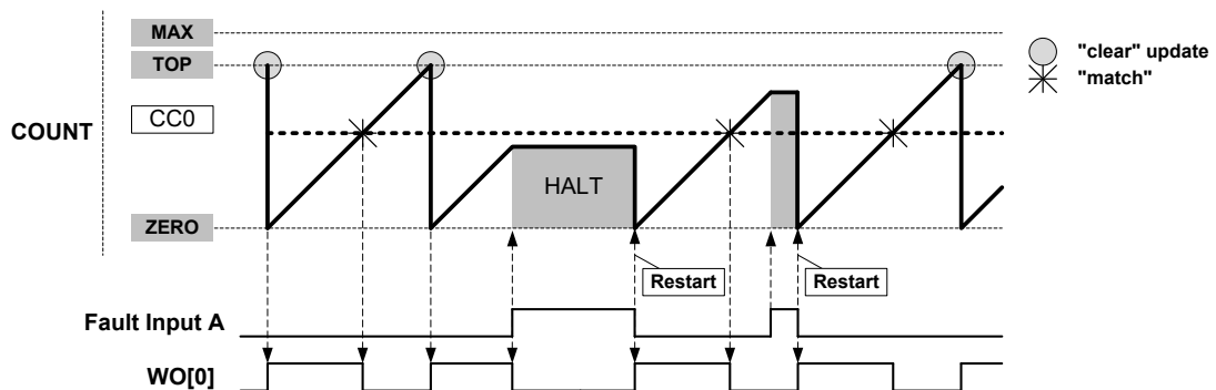
Figure 35-31. Waveform Generation with Fault Qualification, Halt, and Restart Actions
