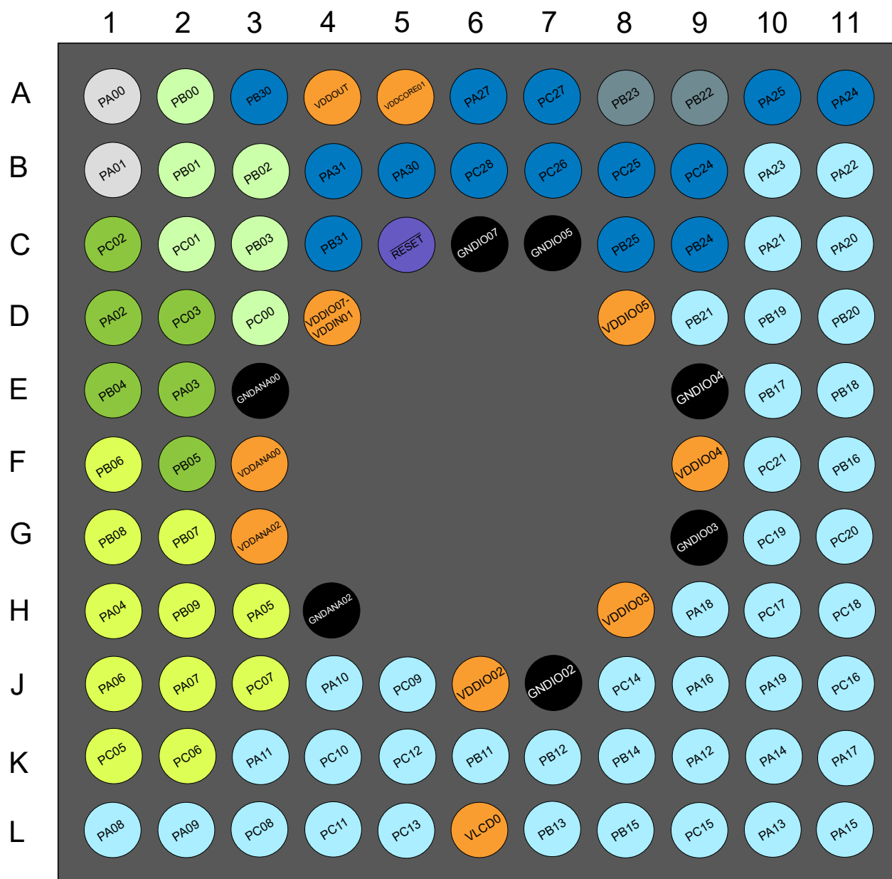
Figure 4-4. UFBGA100
