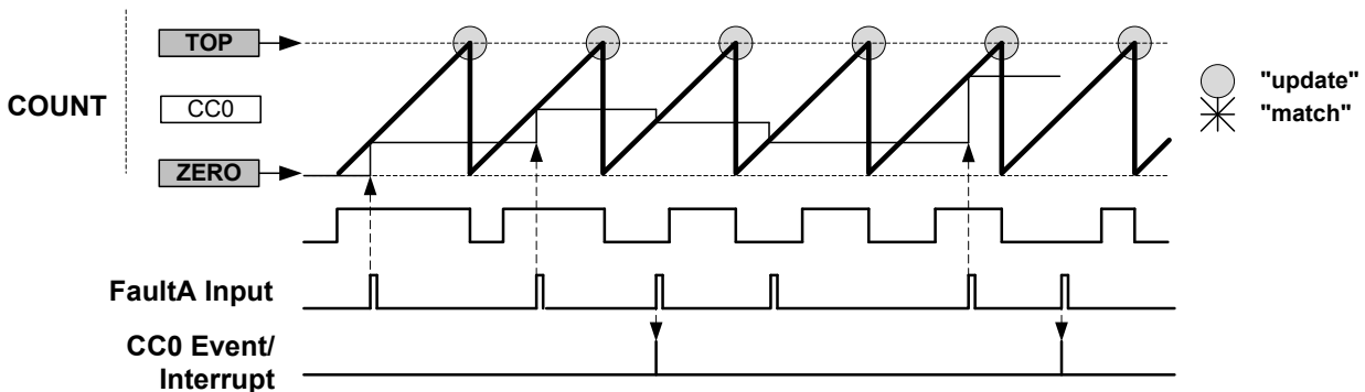
Figure 35-29. Capture Action "DERIVO"
