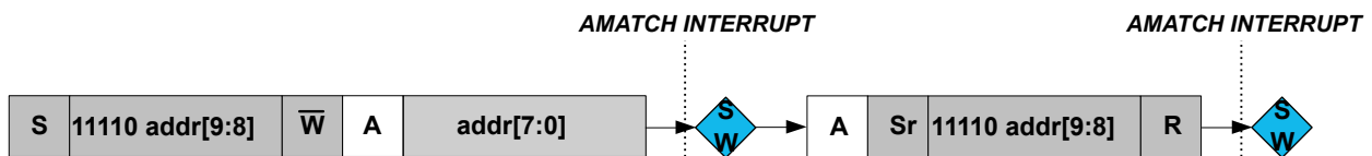
Figure 33-11. 10-bit Addressing
