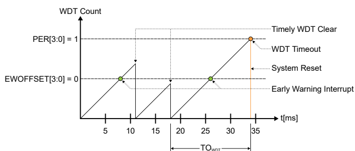
Figure 18-2. Normal-Mode Operation
