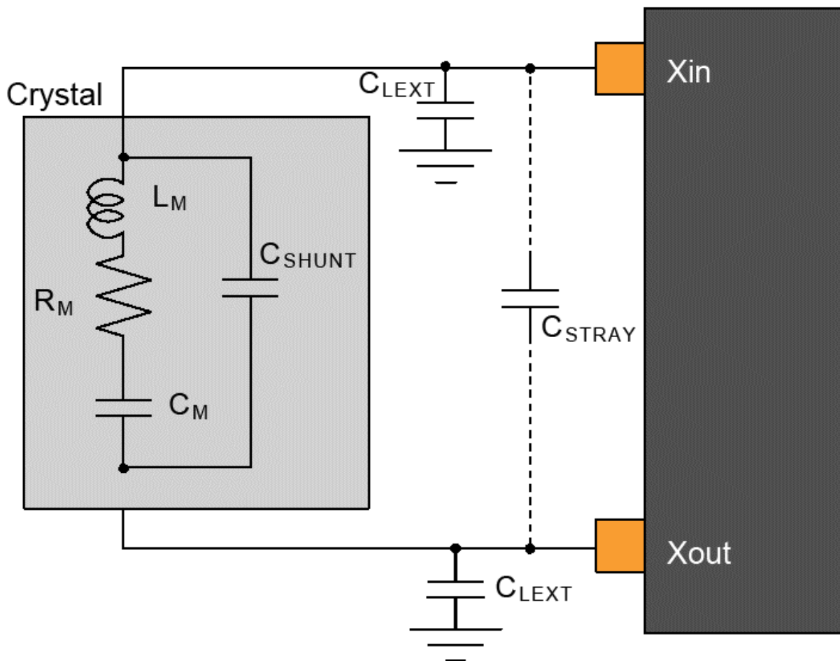
Figure 40-2. Oscillator Connection
