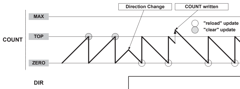
Figure 31-3. Counter Operation
