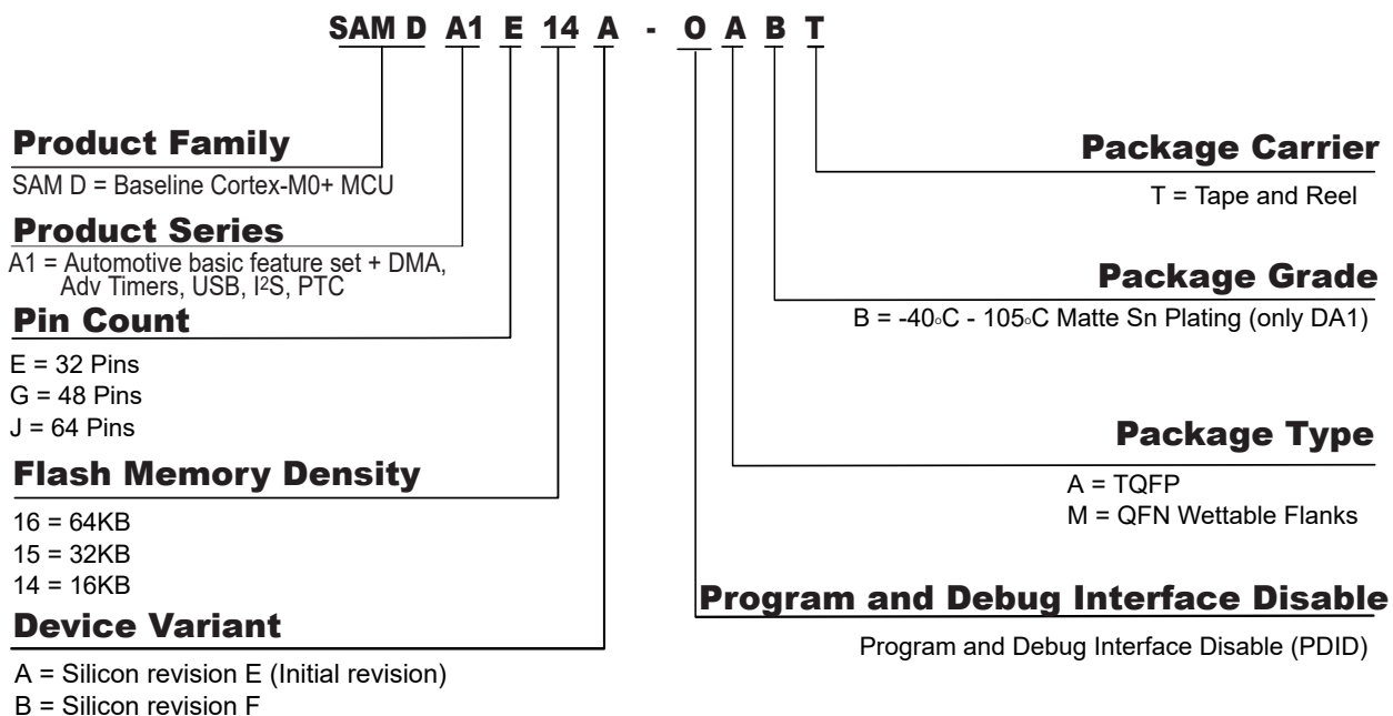
Figure 3-1. SAM DA1 Ordering Information
