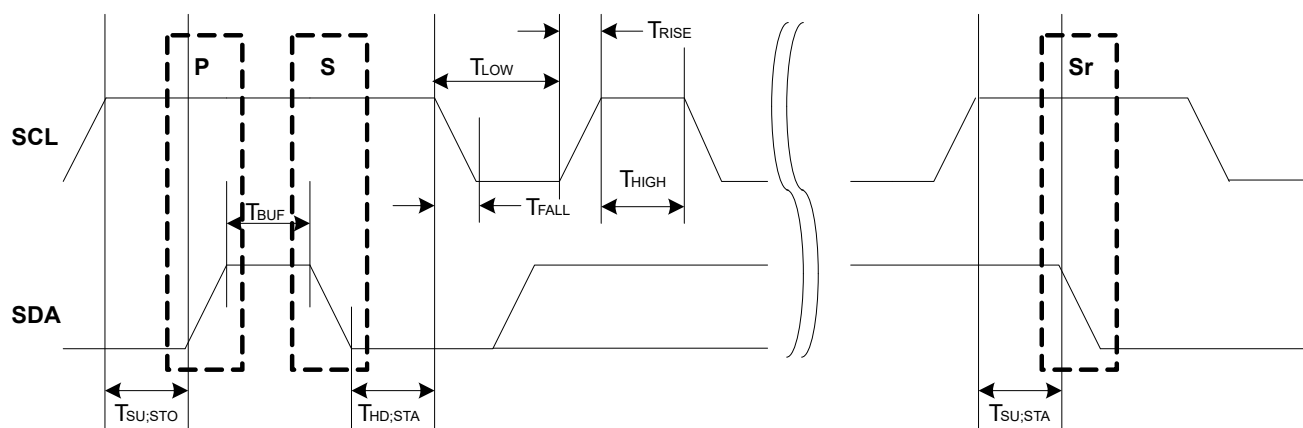
Figure 26-6. SCL Timing
