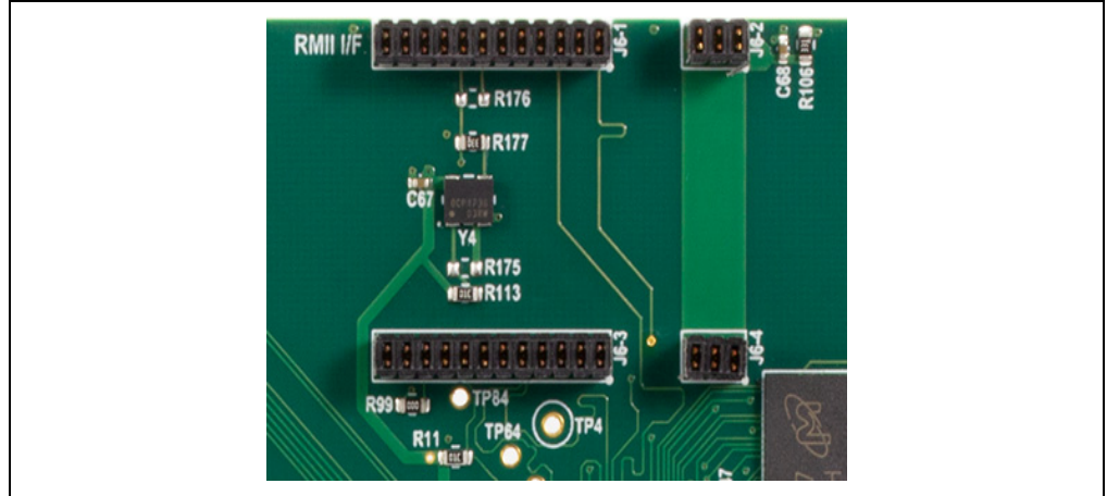
FIGURE 3-4: RMII CONNECTOR
