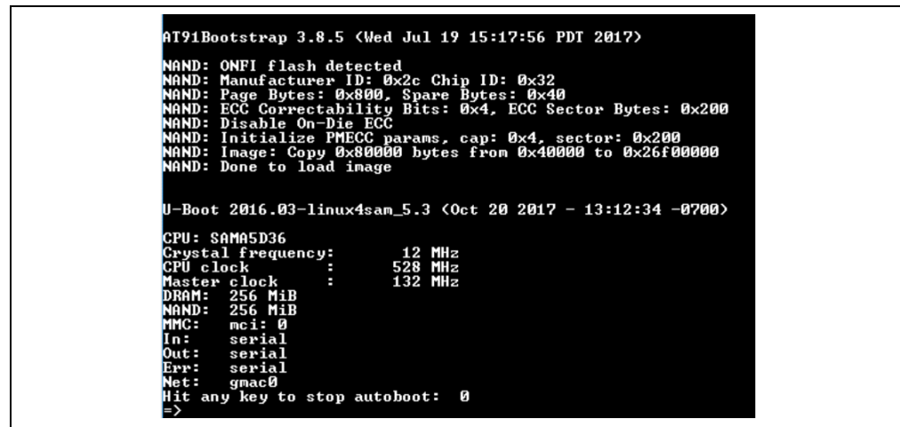
FIGURE 4-5: U-BOOT ENTRY POINT
