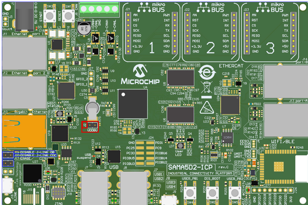
Figure 3-1. Board Overview
