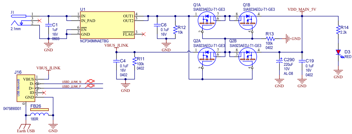
Figure 3-3. Input Powering
