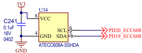
Figure 3-15. ATECC608A-SSHDA Implementation
