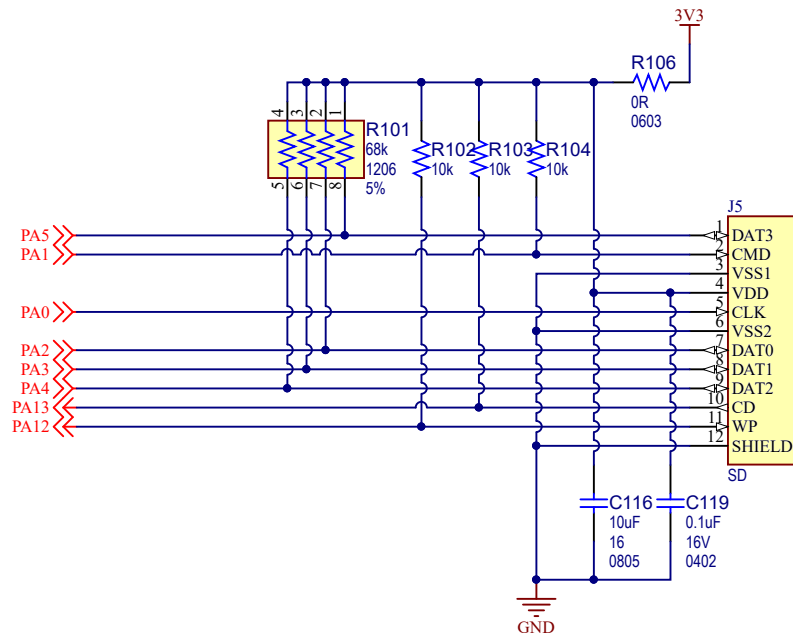
Figure 3-18. SDMMC0 Interface and the Standard SD Socket
