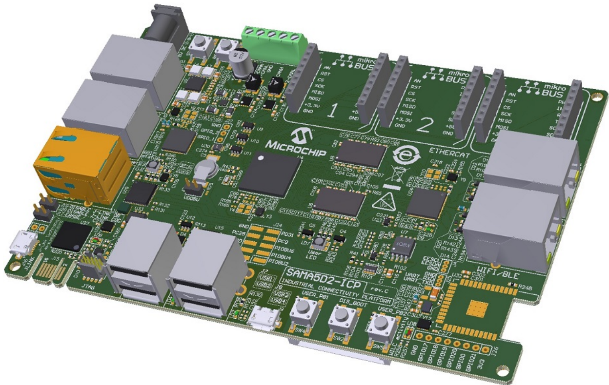
Figure 1. SAMA5D2-ICP Board
