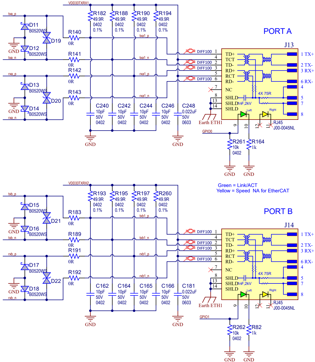
Figure 3-25. EtherCAT Connectors J13 and J14
