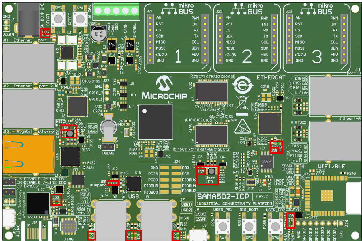
Figure 3-36. On-Board LEDs
