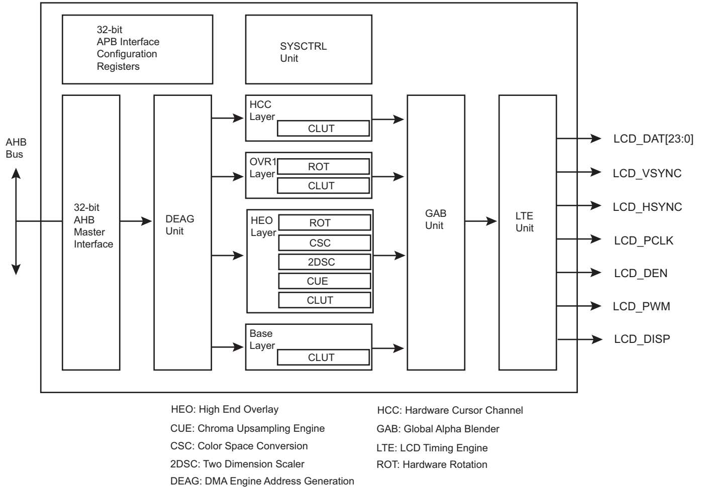
Figure 45-1: Block Diagram
