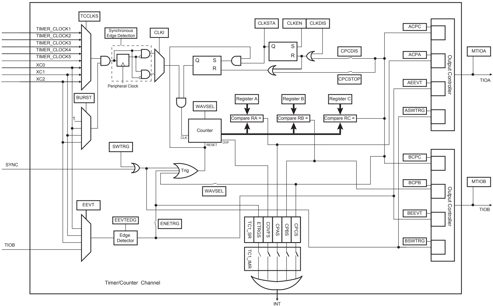
Figure 35-6: Waveform Mode
