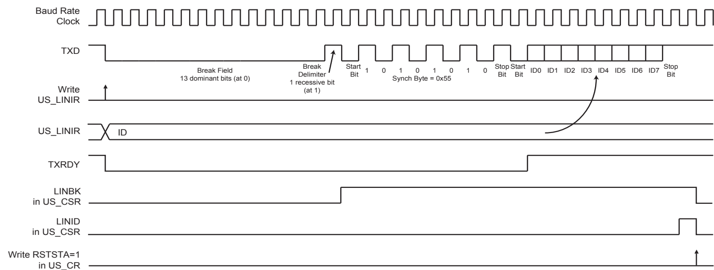
Figure 38-39: Header Transmission
