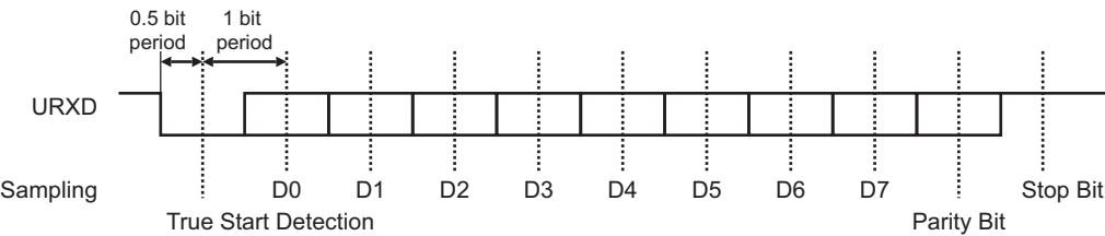
Figure 39-4: Character Reception
