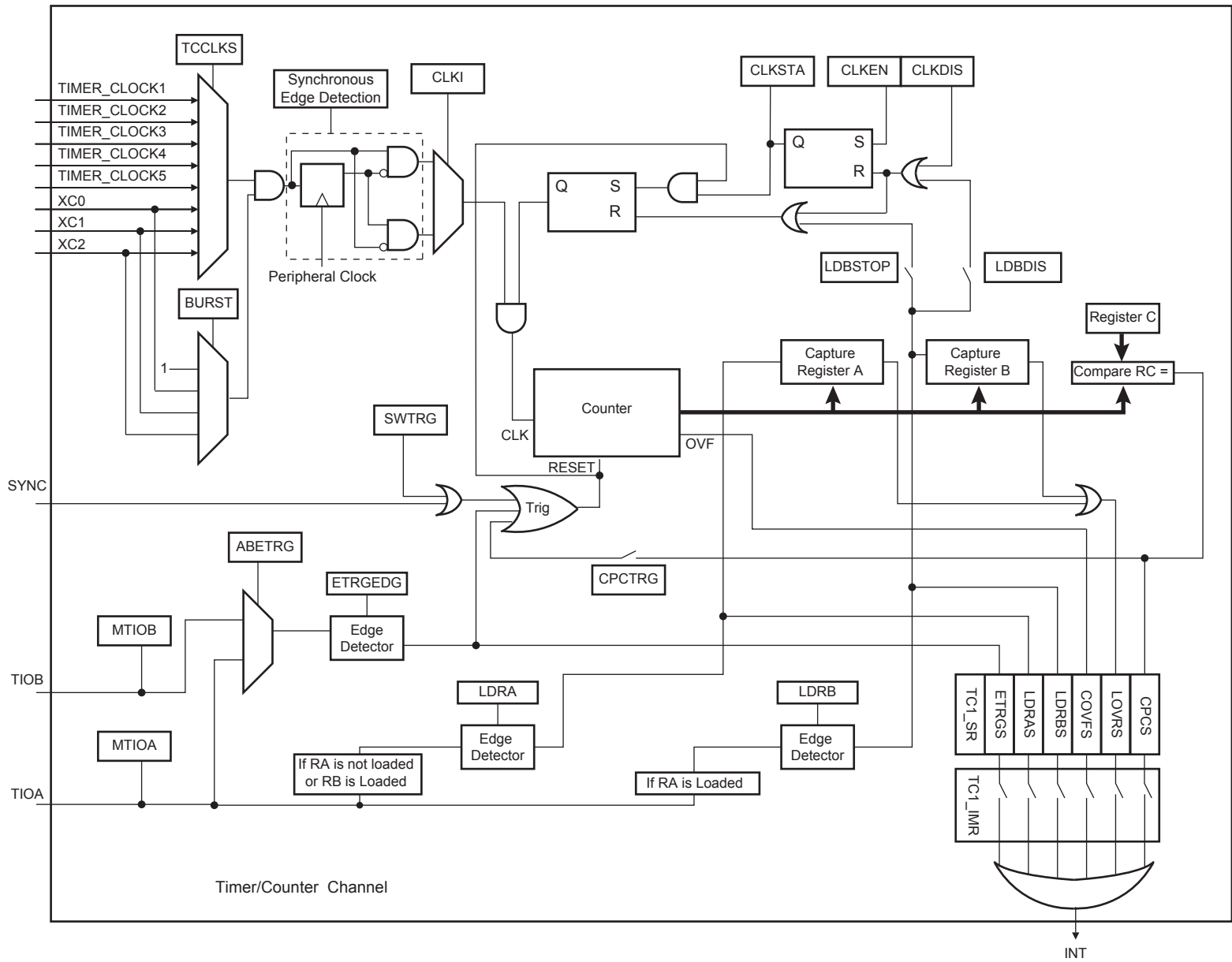
Figure 35-5: Capture Mode
