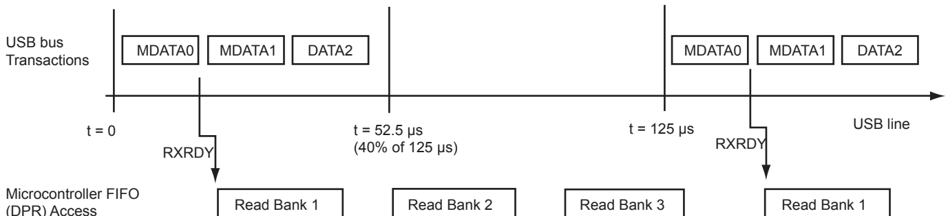
Figure 31-16: Bank Management, Example of Three Transactions per Microframe
