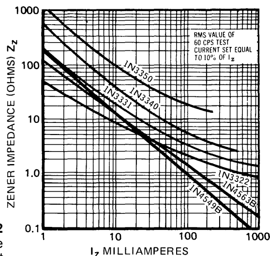
FIGURE 2 Typical Zener Impedance vs. Zener Current
