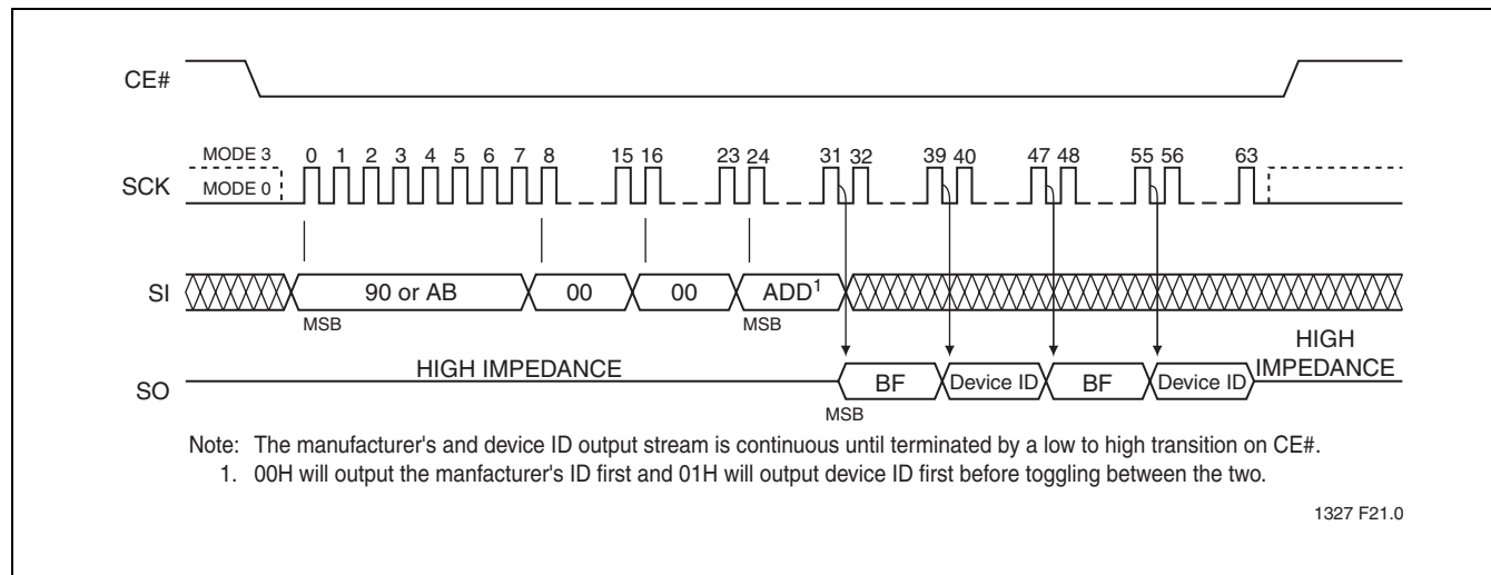
FIGURE 20: Read-ID Sequence
