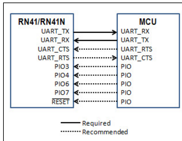
FIGURE 1-1: RN41/RN41N TO MCU INTERFACE
