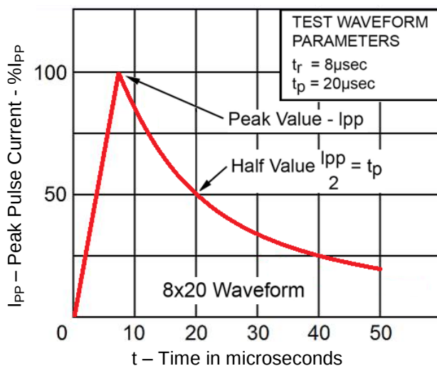
FIGURE 2 Pulse Waveform
