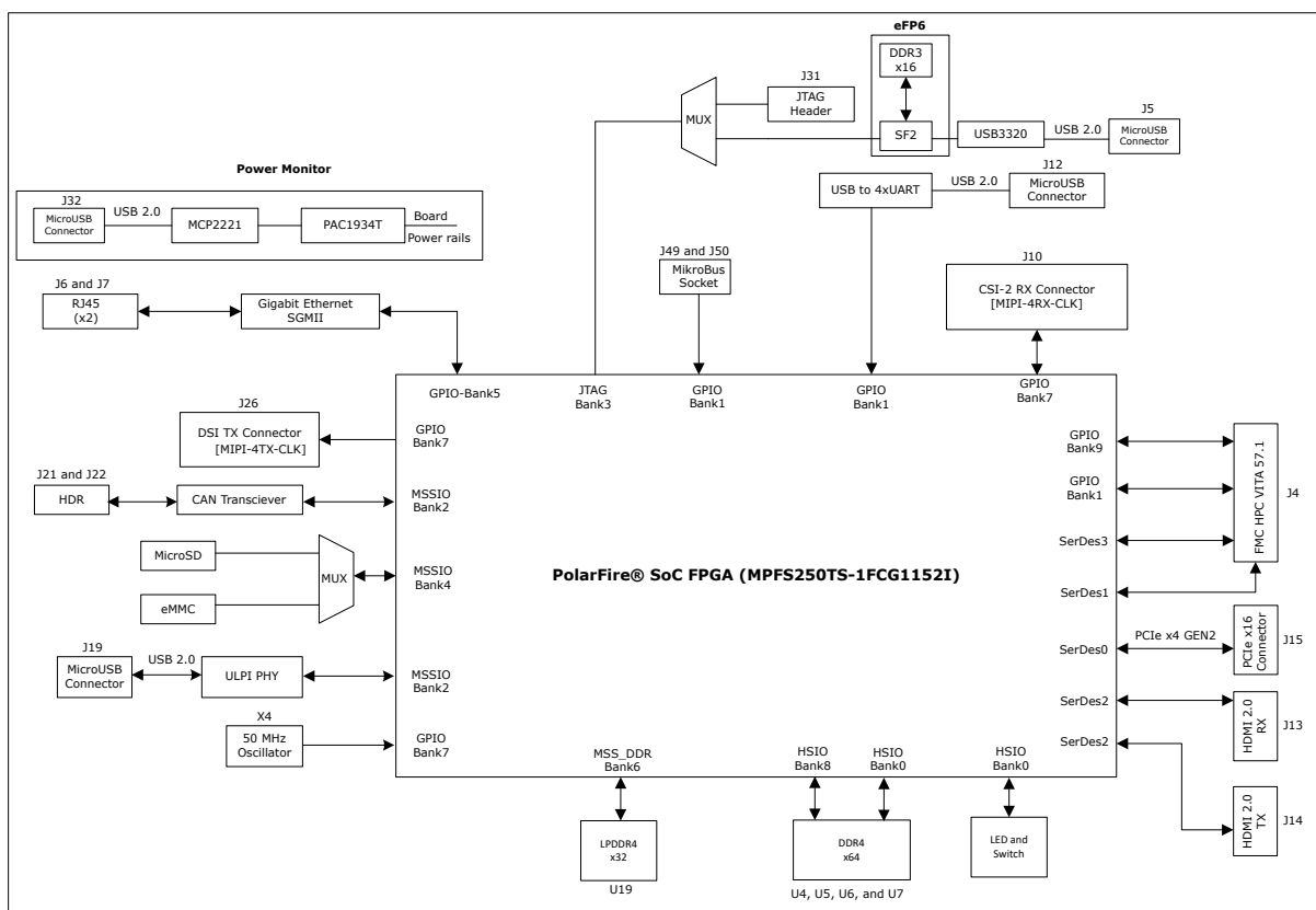
Figure 1-1. Block Diagram
