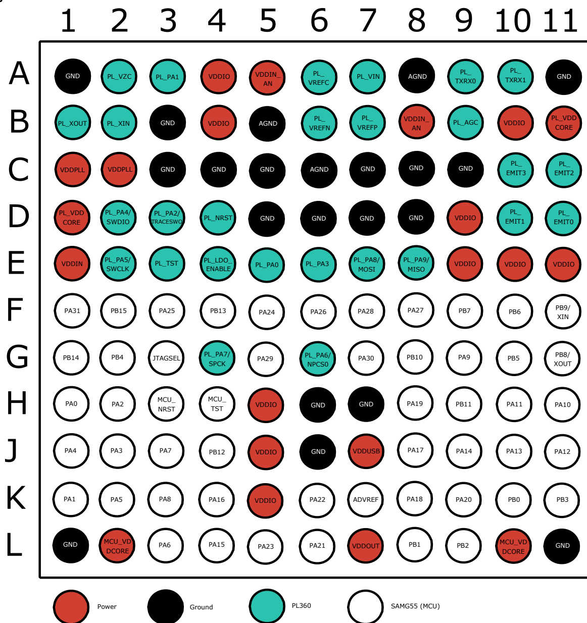
Figure 5-1. PL485 Ballout
