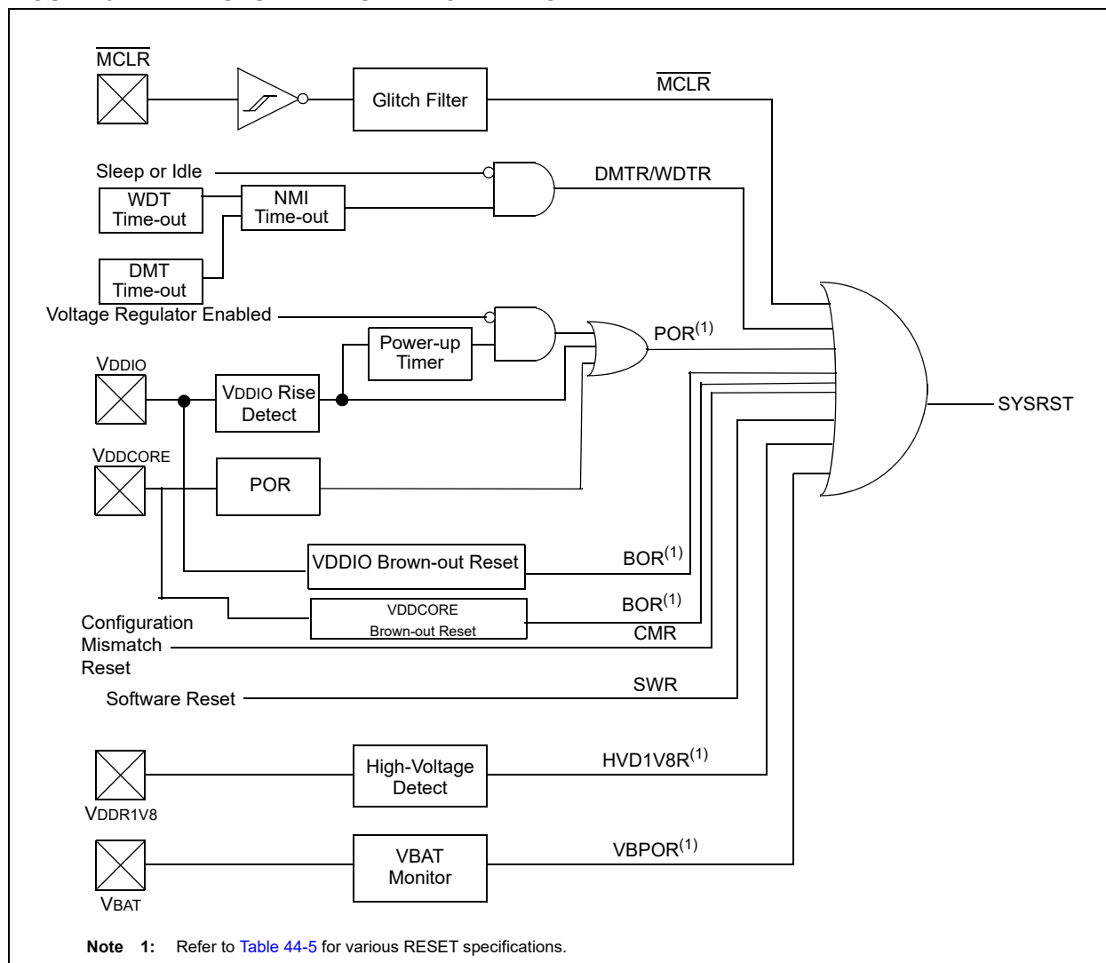
FIGURE 6-1: SYSTEM RESET BLOCK DIAGRAM
