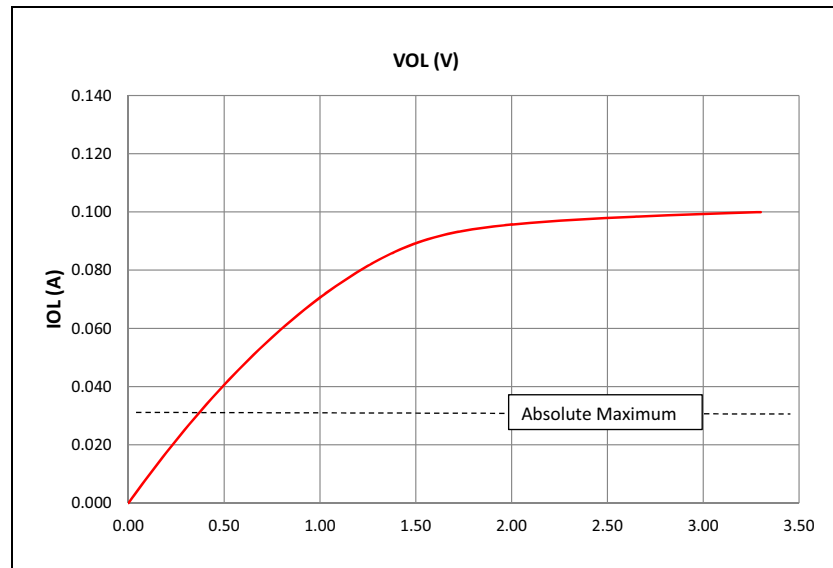
FIGURE 45-6: V_{OL} – 12x DRIVER PINS
