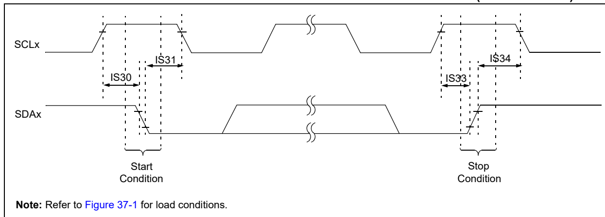
FIGURE 37-18: I2Cx BUS START/STOP BITS TIMING CHARACTERISTICS (CLIENT MODE)
