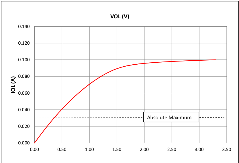
FIGURE 40-6: V_{OL} – 12x DRIVER PINS
