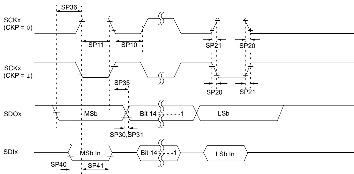
FIGURE 37-11: SPIx MODULE HOST MODE (CKE = 1) TIMING CHARACTERISTICS
