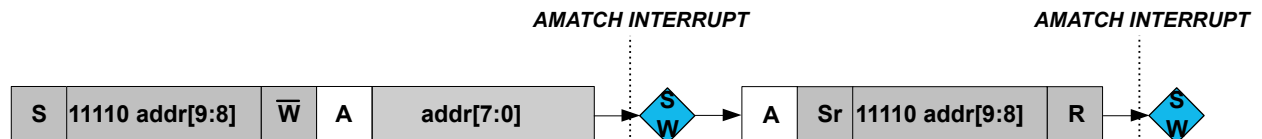
Figure 32-12. 10-bit Addressing
