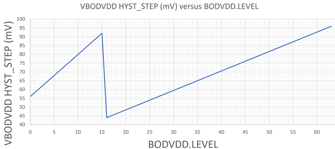
Figure 46-1. VBODVDDHYST_STEP Graph
