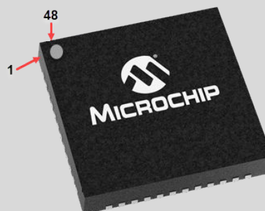
Figure 4-2. VQFN
