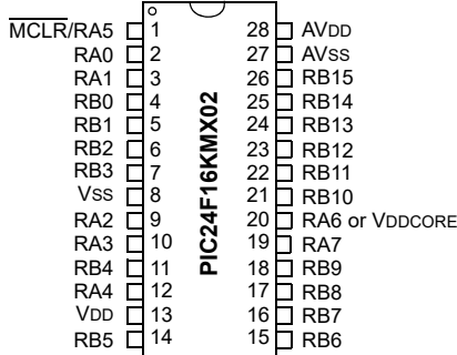
28-Pin SPDIP/SSOP/SOIC
