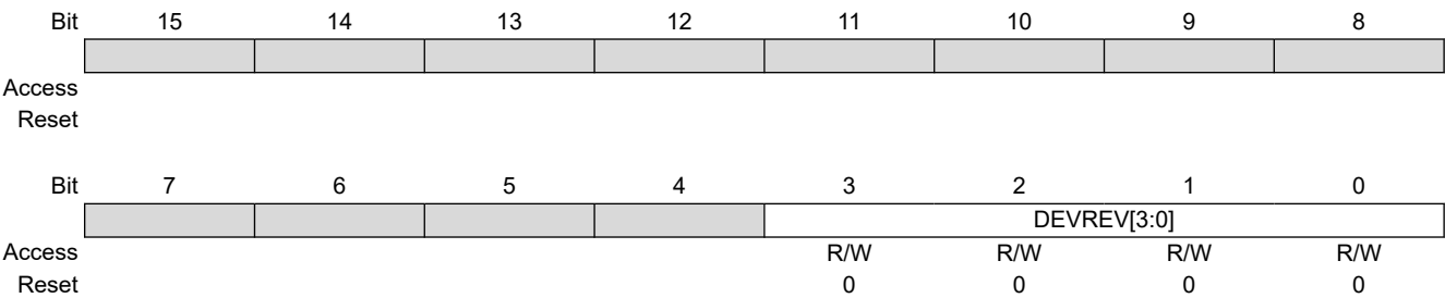
Bits 3:0 – DEVREV[3:0] Device Revision bits
