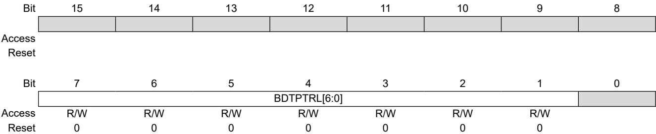
Bits 7:1 – BDTPTRL[6:0] BDT Address Low bits
