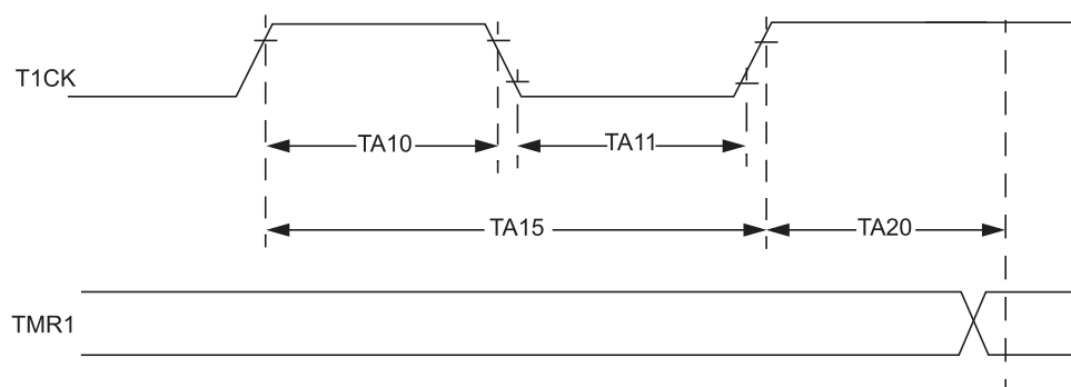
Figure 32-5. Timer1 External Clock Timing Characteristics
