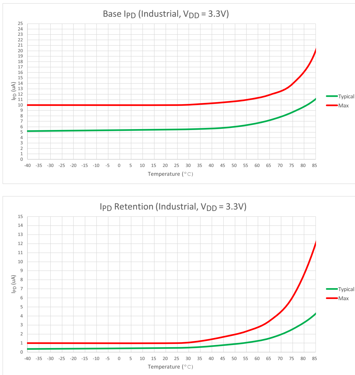
FIGURE 30-3: I_{PD} VS. TEMPERATURE GRAPHS (PAGE 2 OF 2) (1,2)
