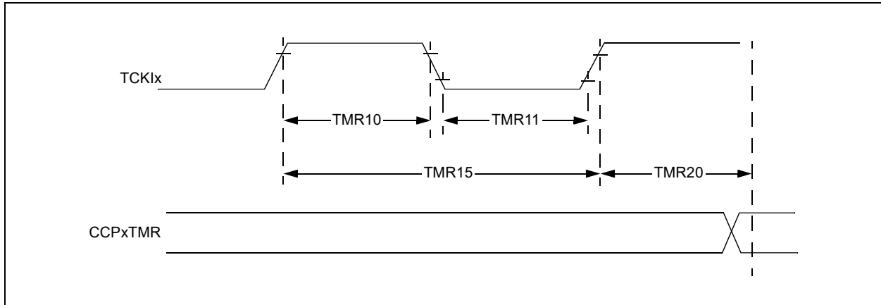
FIGURE 30-13: MCCP TIMER MODE EXTERNAL CLOCK TIMING CHARACTERISTICS
