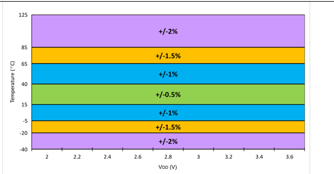
FIGURE 30-10: FRC ACCURACY OVER TEMPERATURE AND V_{DD}^{(1)}
