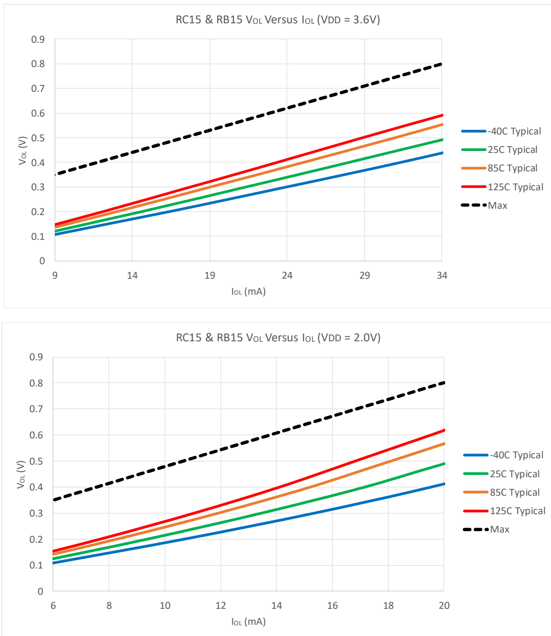
FIGURE 30-6: RC15, RB15 V_{OL} VS. I_{OL} CHARACTER GRAPHS (1)
