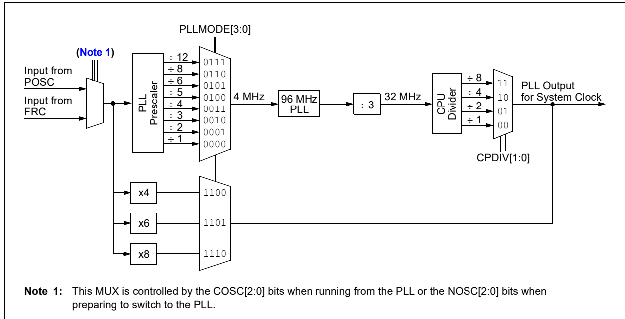
FIGURE 9-2: PLL BLOCK
