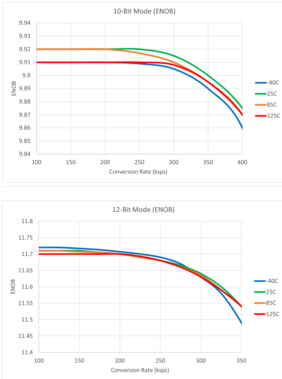
FIGURE 30-24: 10-BIT AND 12-BIT ENOB
