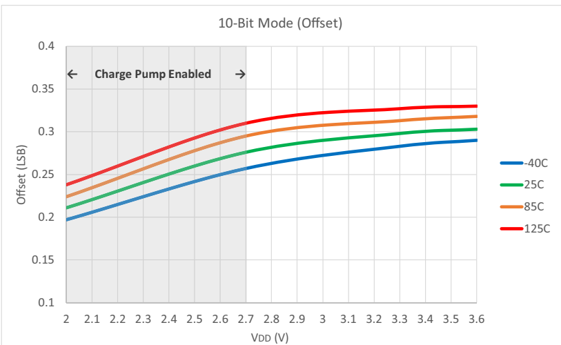
FIGURE 30-27: GAIN AND OFFSET VOLTAGES
