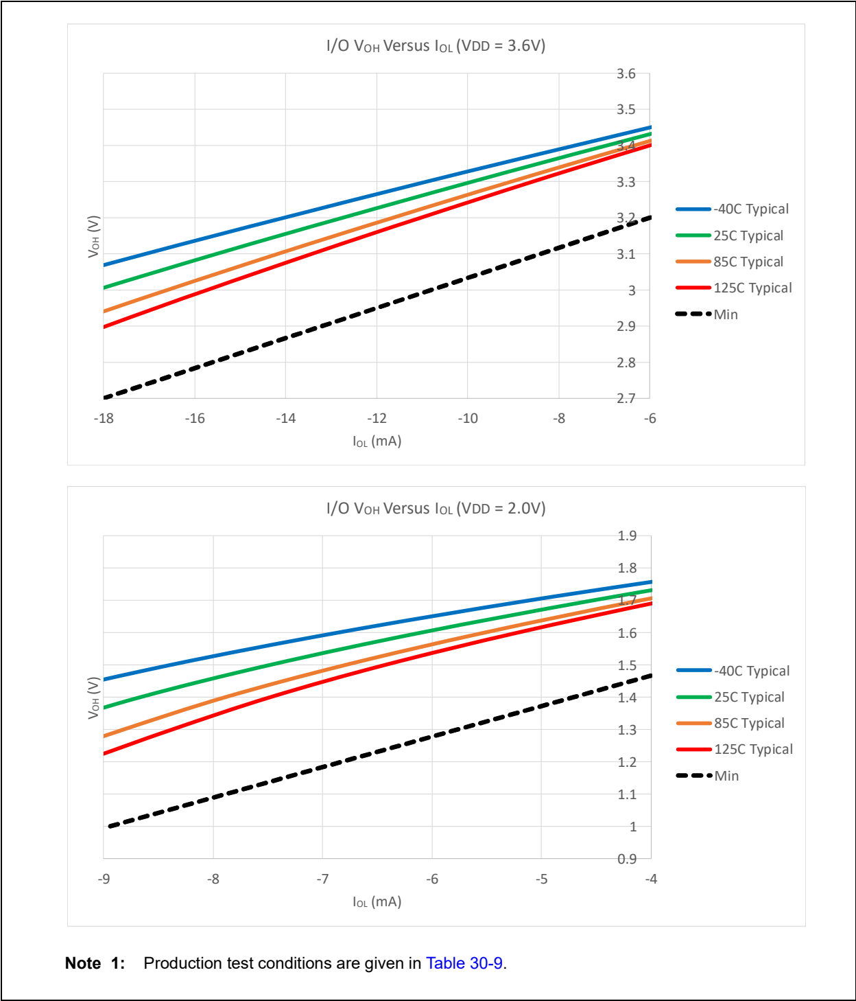
FIGURE 30-5: I/O V OH VS. I OL CHARACTER GRAPHS (1)
