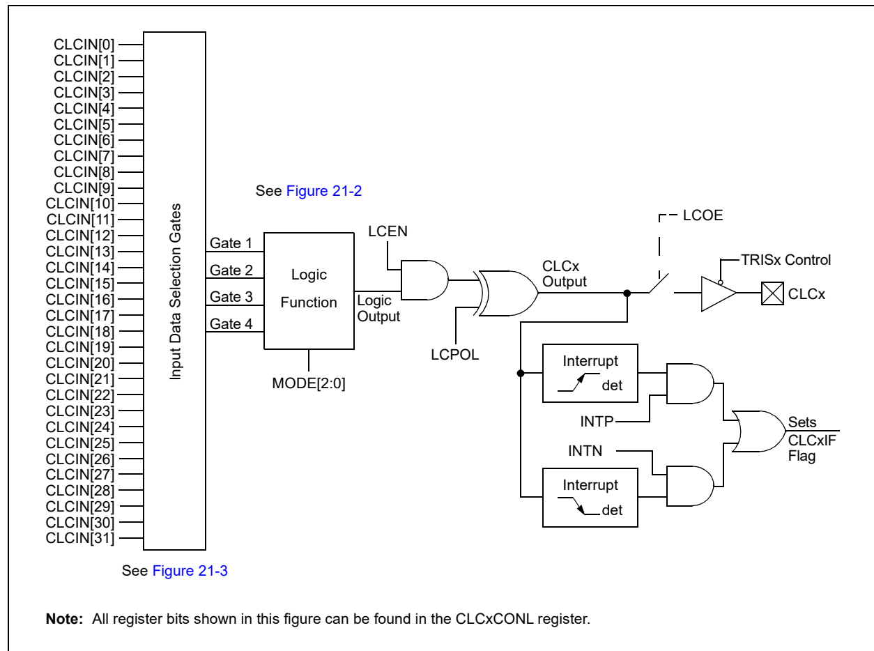
FIGURE 21-1: CLCx MODULE
