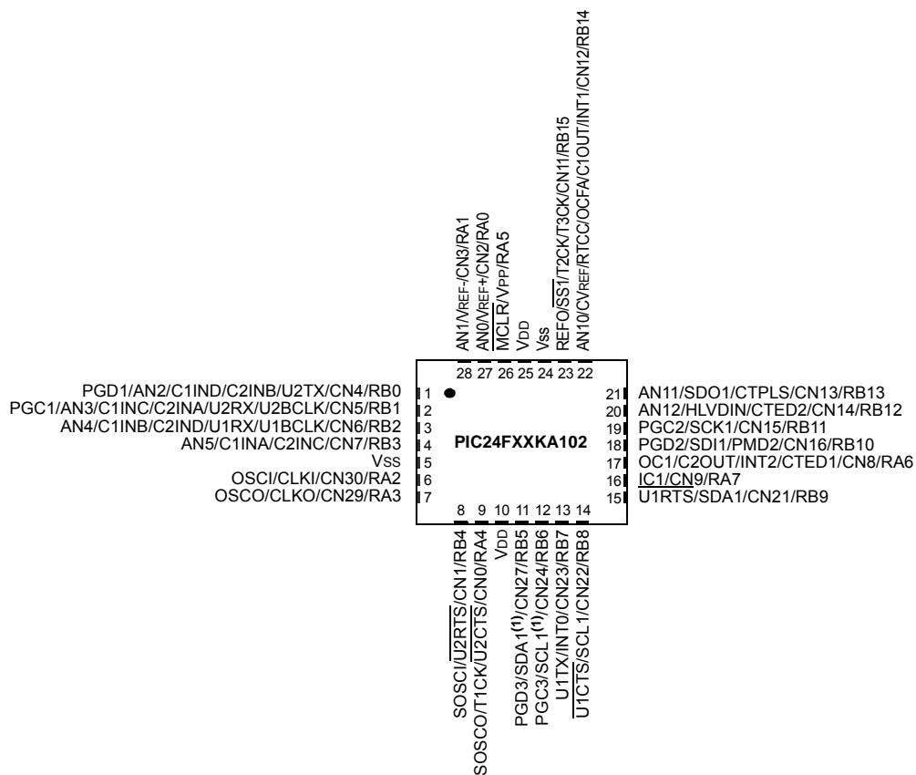
28-Pin QFN (2,3)
