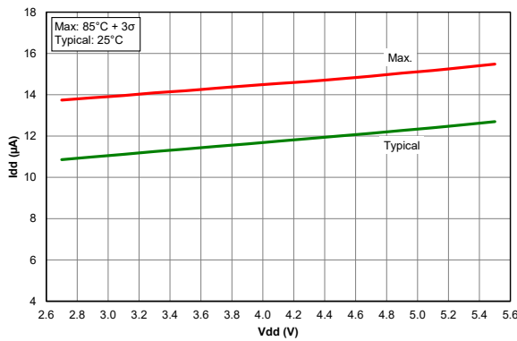
Figure 39-68. I_{PD} , Low-power Brown-out Reset, LPBOR = 0, PIC18F26/45/46K40 only
