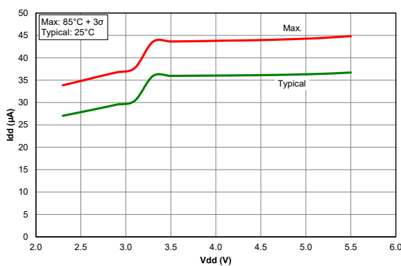
Figure 39-70. I_{PD} , Comparator, PIC18F26/45/46K40 only
