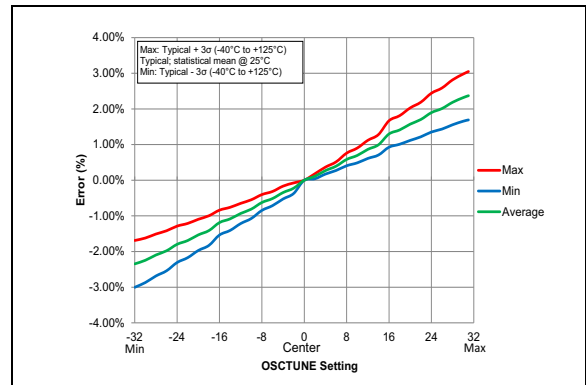
FIGURE 45-123: OSCUNE Center Frequency, PIC18LF24/25K42 Only.
