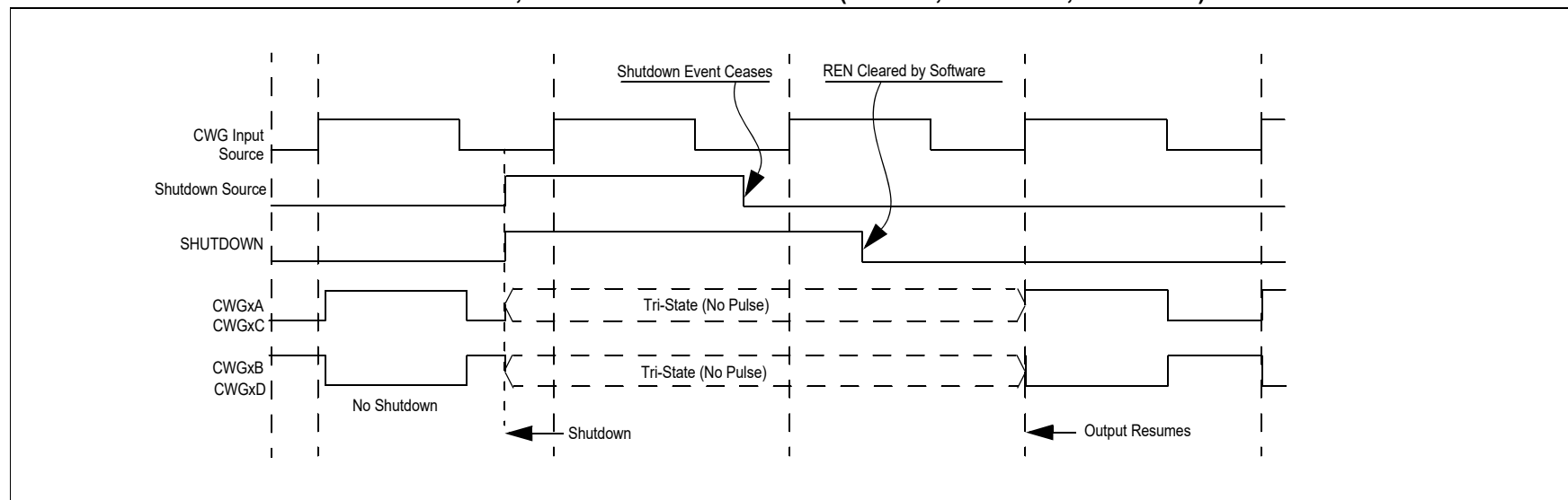
FIGURE 26-15: SHUTDOWN FUNCTIONALITY, AUTO-RESTART DISABLED (REN = 0, LSAC = 01, LSB0 = 01)
