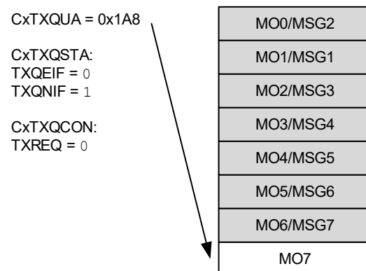
Figure 38-36. TXQ - Next Six Messages Loaded
